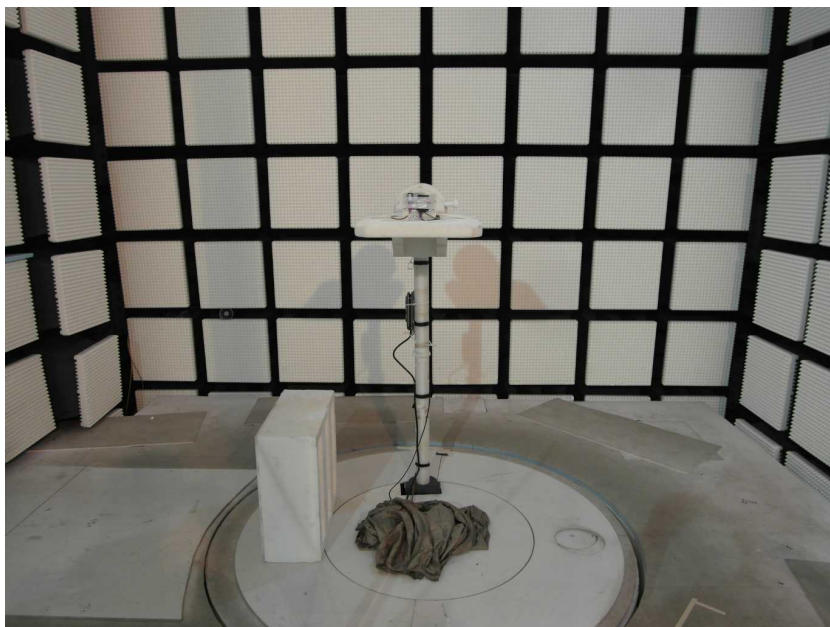
Photo 4: EUT at the anechoic chamber, test setup valid for all three antennas
