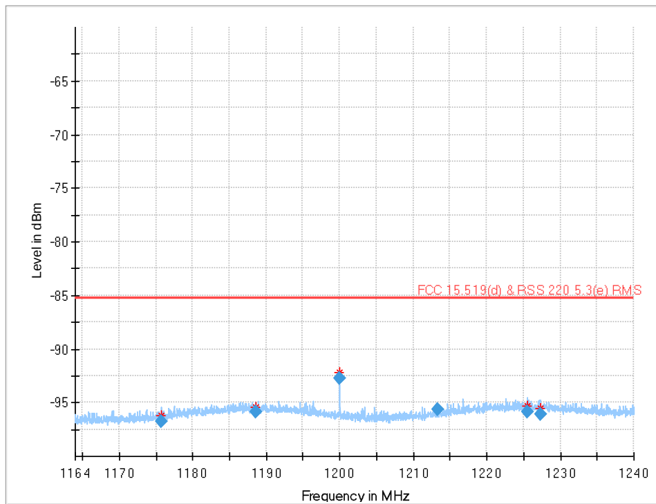
Plot 25: 1164 MHz to 1240 MHz (§15.519 (d)), UWB test mode, DUT-A, CH5
