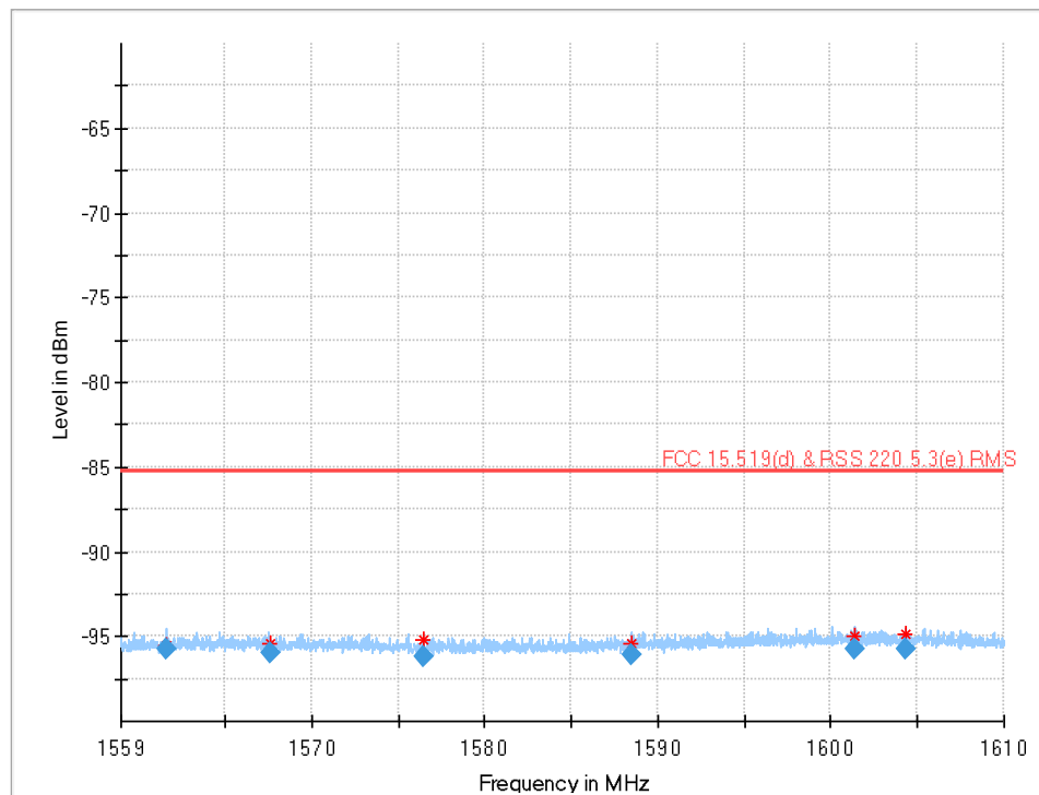
Plot 28: 1559 MHz to 1610 MHz (§15.519 (d)), UWB test mode, DUT-A, CH9
