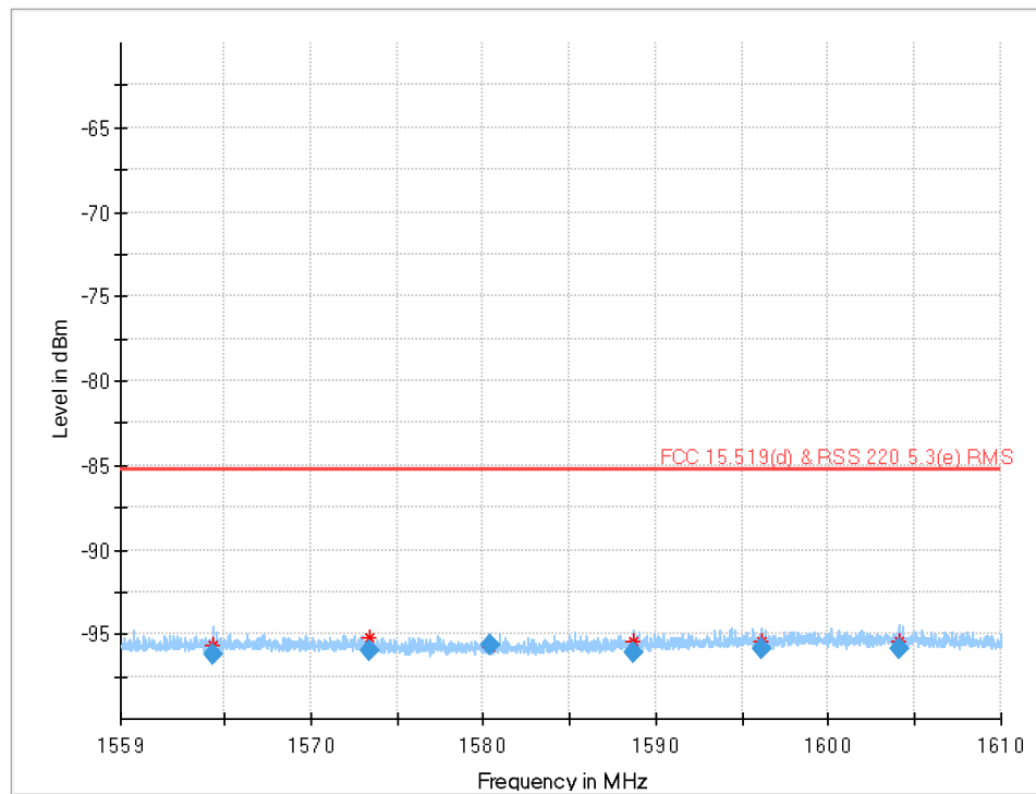
Plot 27: 1559 MHz to 1610 MHz (§15.519 (d)), UWB test mode, DUT-A, CH5
