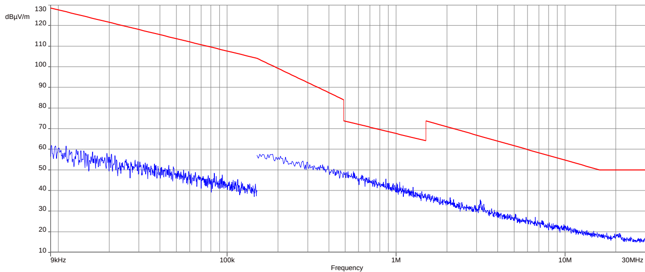
Plot 1: 9 kHz to 30 MHz, 2402 MHz, transmit mode, valid for 2 Msps and 1 Msps
