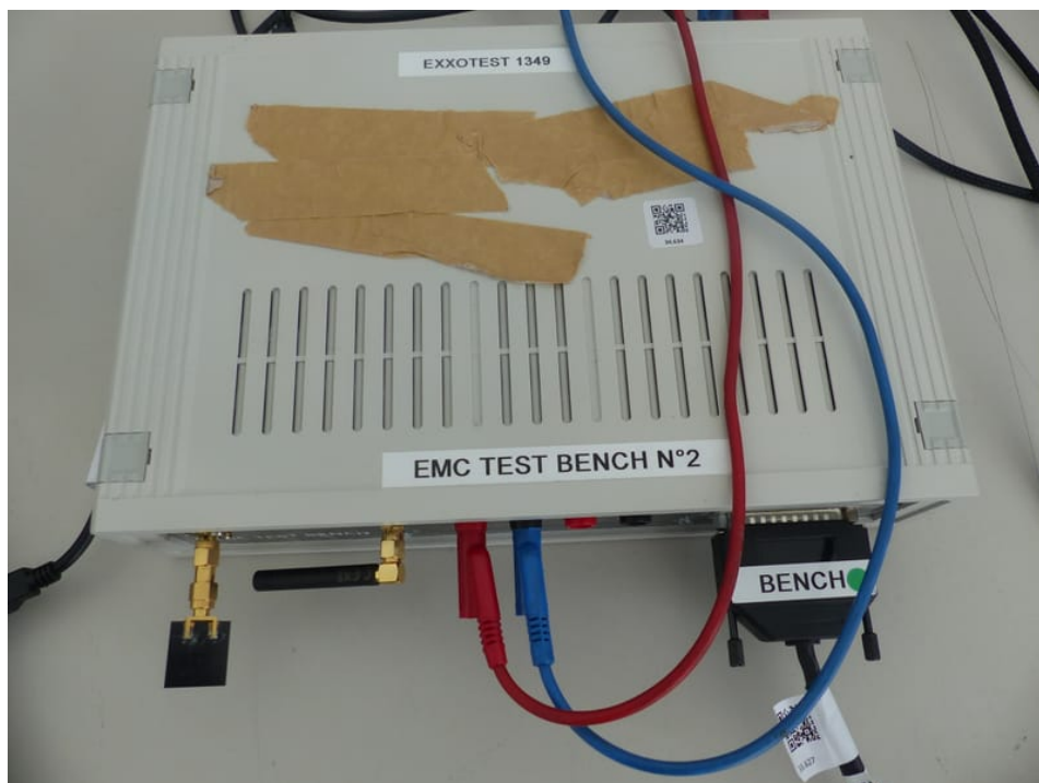
Photo 14: AE2: "EMC Test Bench N°2"
