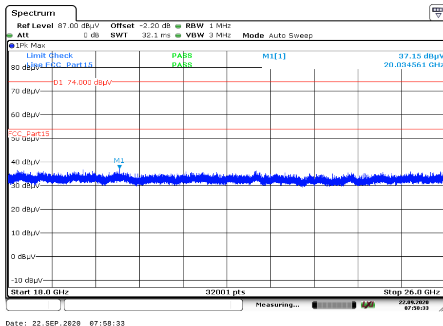
Plot 4: 18 GHz to 26 GHz, mid channel, vertical & horizontal polarization, GFSK
