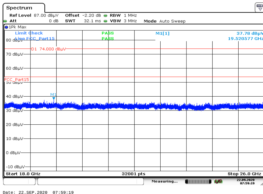
Plot 6: 18 GHz to 26 GHz, high channel, vertical & horizontal polarization, CW
