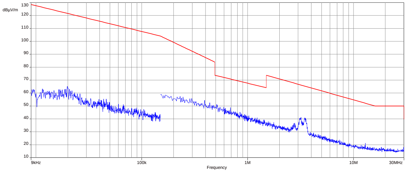
Plot 1: 9 kHz to 30 MHz, low channel, GFSK
