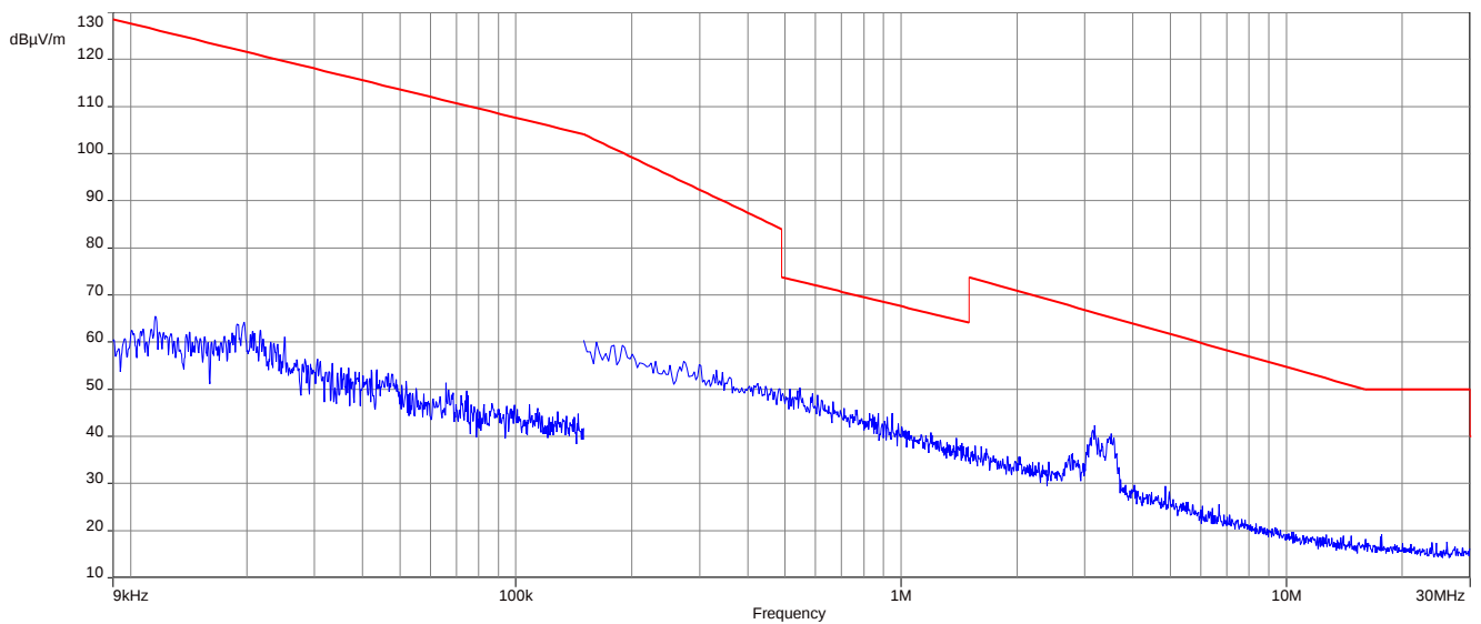
Plot 2: 9 kHz to 30 MHz, mid channel, GFSK
