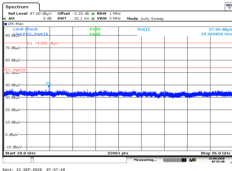
Plot 4: 18 GHz to 26 GHz, mid channel, vertical & horizontal polarization, CW
