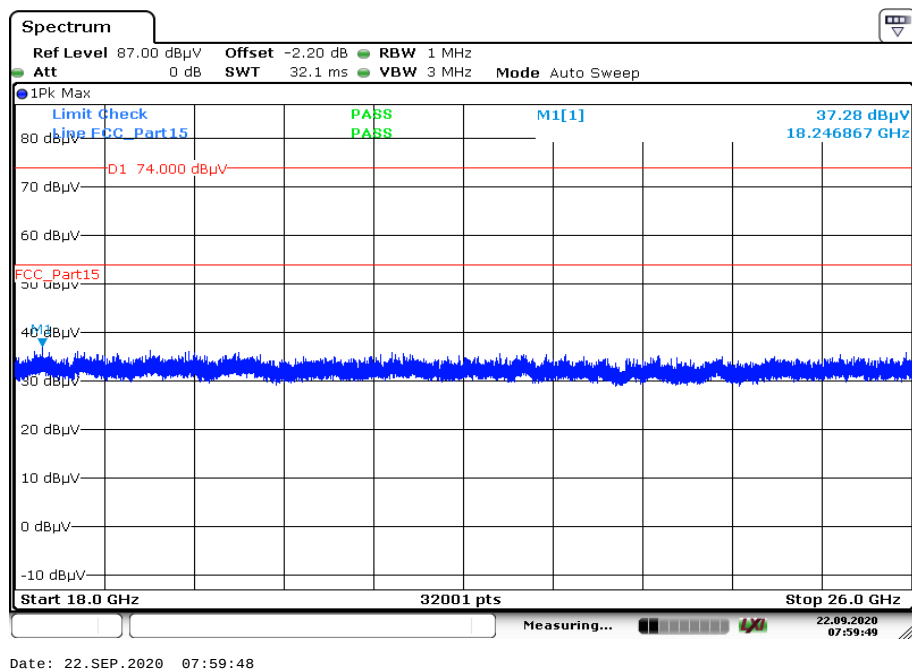
Plot 6: 18 GHz to 26 GHz, high channel, vertical & horizontal polarization, GFSK
