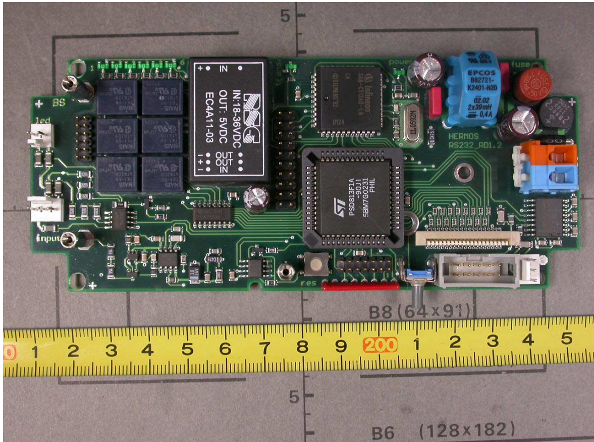
Top view – Main board
