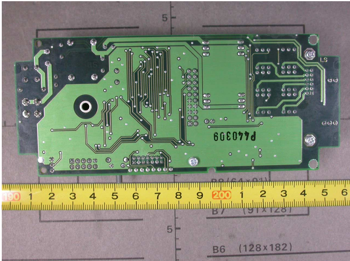
Bottom view – Main board
