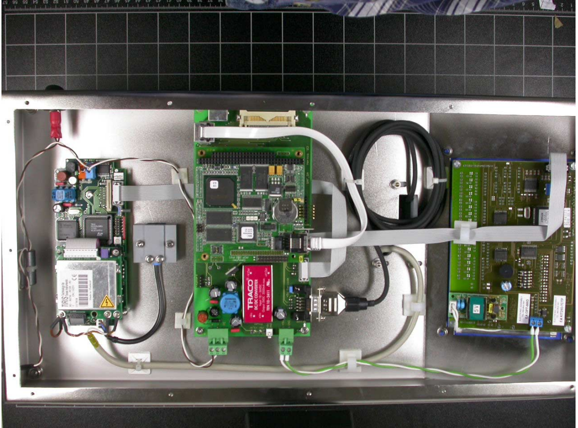
Unit disassembled
