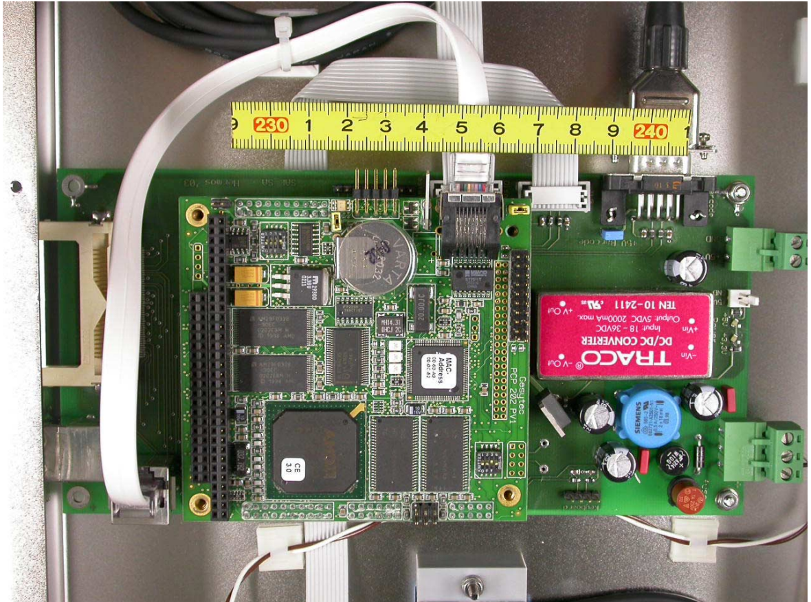
Top view – Processor board
