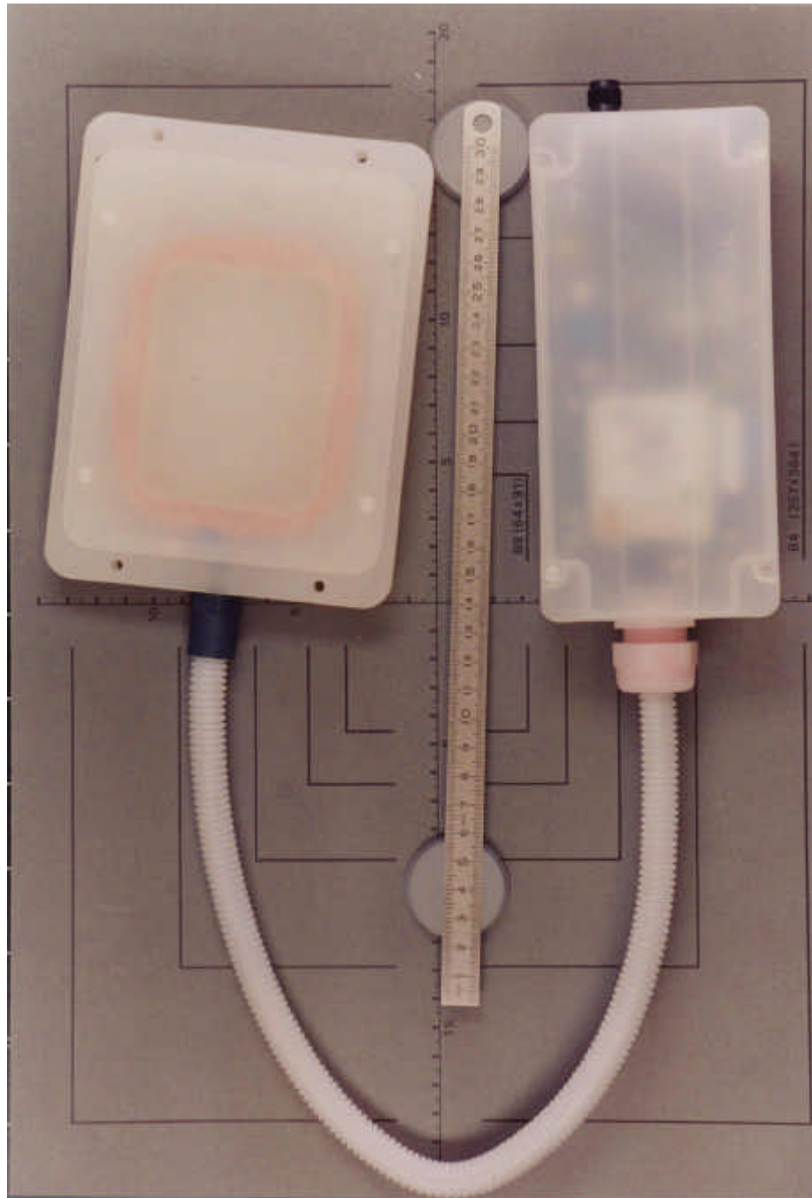
Top view of transponder reader system
