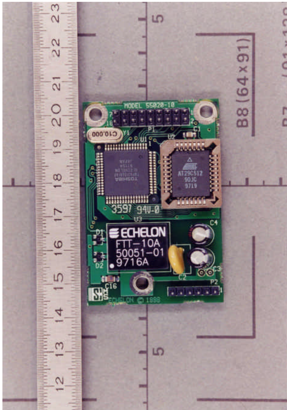
Top view of printed board of flash control module
