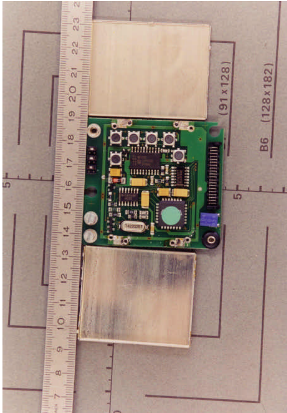
Top view of disassembled RF module
