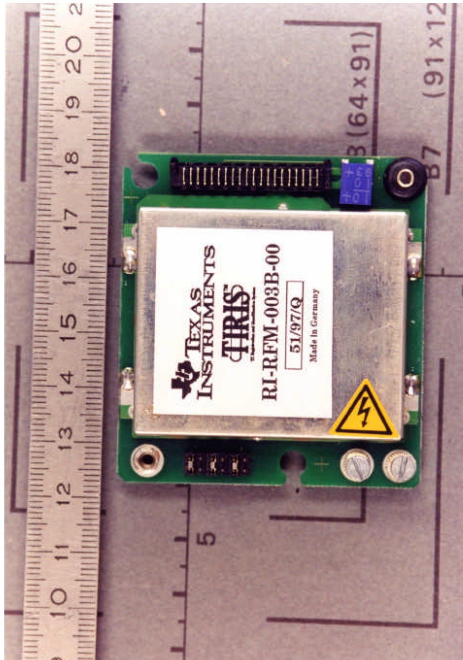
Top view of printed board of RF module
