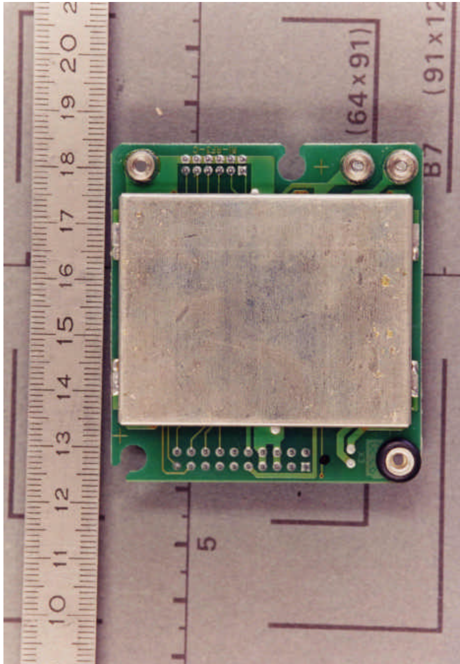
Bottom view of printed board of RF module
