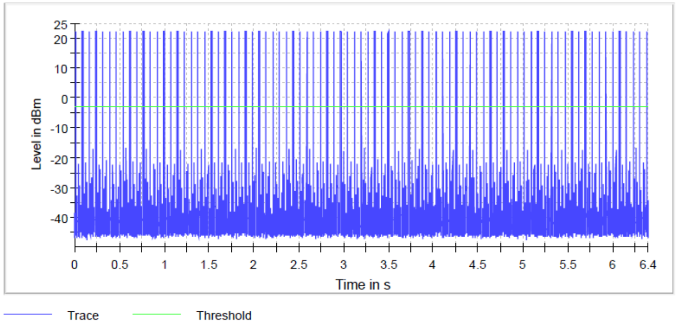
Figure 35: Time of channel occupancy LOW channel
