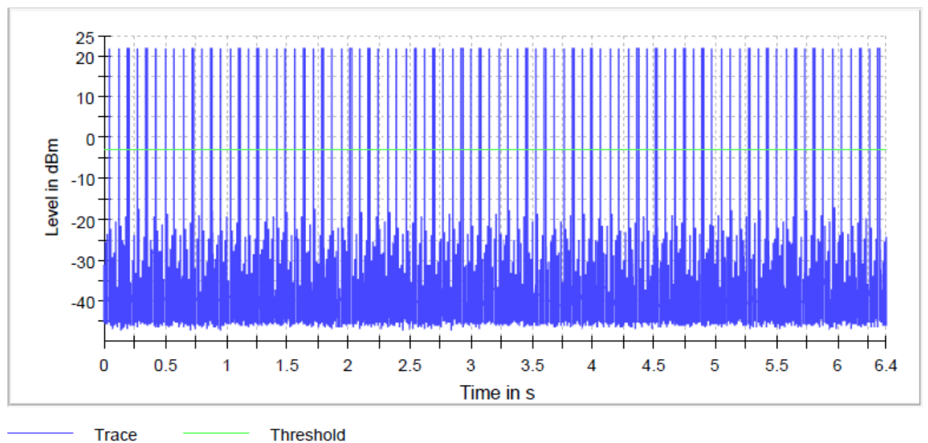
Figure 36: Time of channel occupancy MID channel
