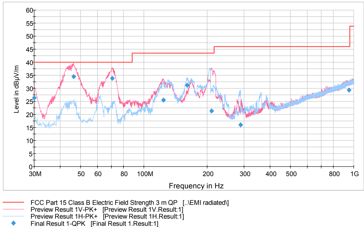
Figure 2. Measured curve with peak-detector. Channel MID.
