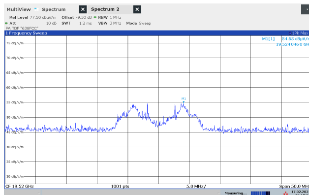
Emissions 19520 MHz, 2440 MHz, GFSK, HP @1m, M70XC Ant
