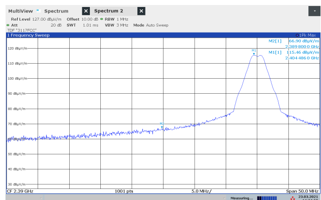
Band Edge 2405 MHz, GFSK, Peak, PowLev 220, Ext Whip Ant
