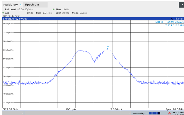
Emissions 7320 MHz, 2440 MHz, GFSK, VP, M70XC Ant
