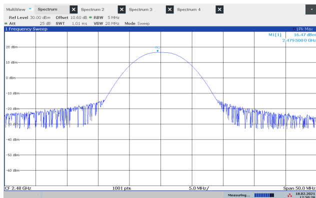
Peak Power, 2480 MHz, PLev 220
