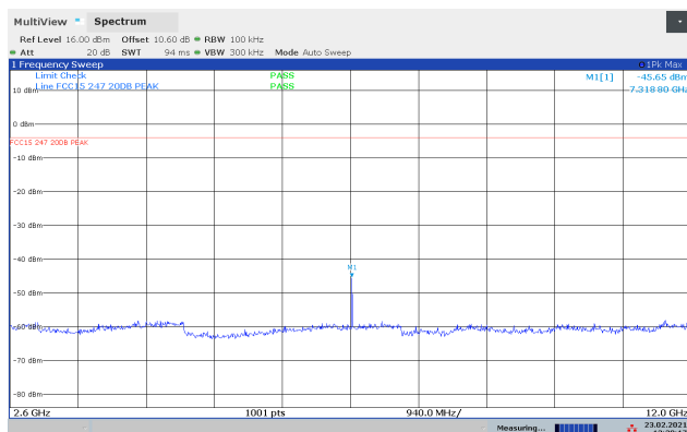
Conducted Emissions 2600-12000 MHz, 2440 MHz, PLev 236
