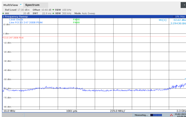
Conducted Emissions 10-2300 MHz, 2405 MHz, PLev 236
