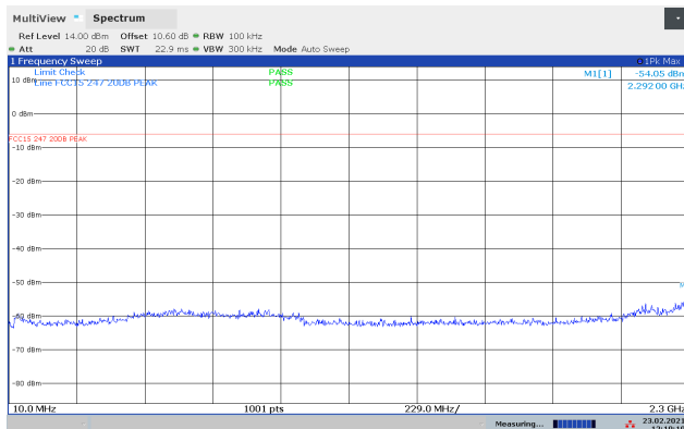
Conducted Emissions 10-2300 MHz, 2480 MHz, PLev 236
