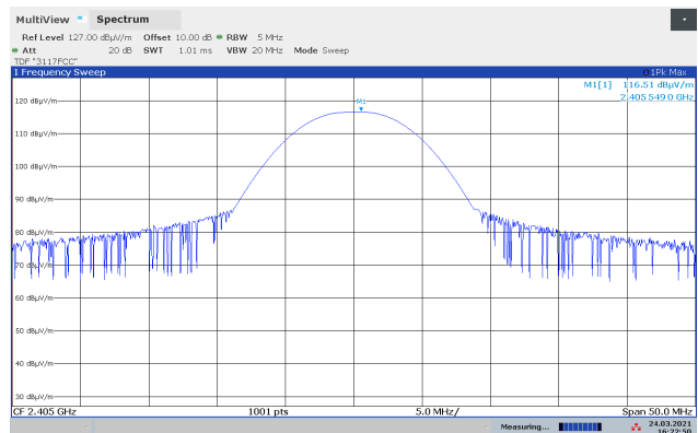
Maximum Field Strength, 2405 MHz, PLev 220, External Whip Ant
