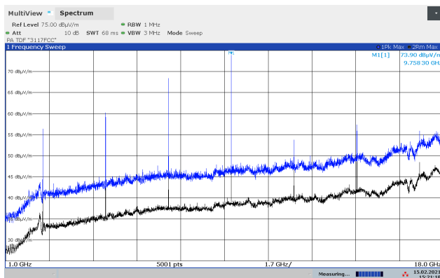
Radiated Emissions 1 - 18 GHz, 2440 MHz, HP, M70XC Ant
