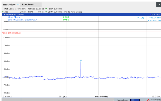
Conducted Emissions 2600-12000 MHz, 2405 MHz, PLev 236
