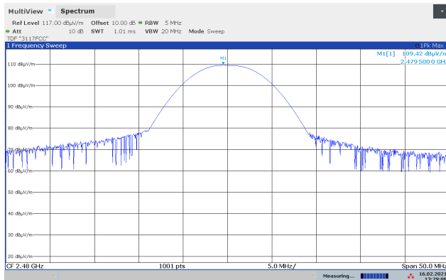
Maximum Field Strength, 2480 MHz, PLev 220, M70XC
