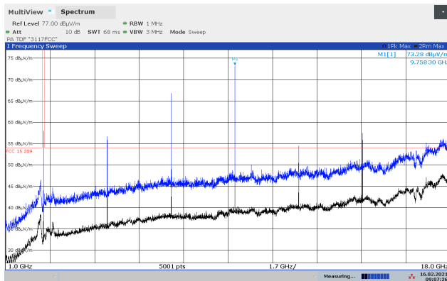
Radiated Emissions 1 - 18 GHz, 2440 MHz, HP, Int F-Ant
