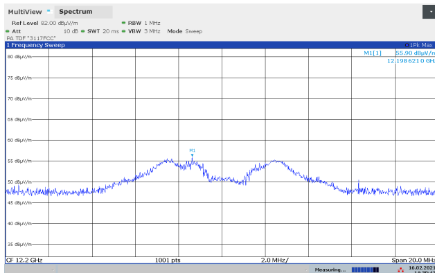
Emissions 12200 MHz, 2440 MHz, GFSK, HP, M70XC Ant
