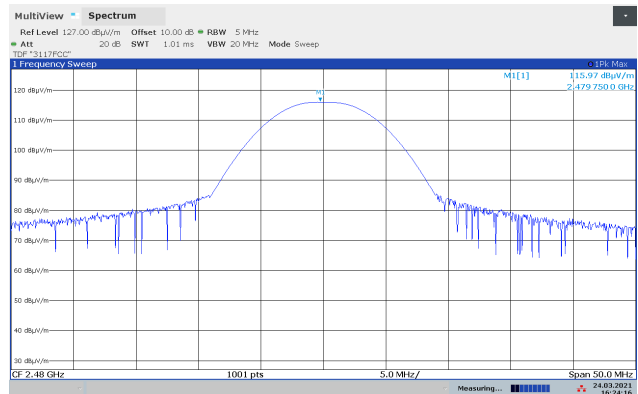
Maximum Field Strength, 2480 MHz, PLev 220, External Whip Ant
