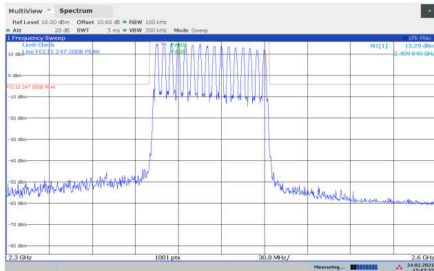
Conducted Emissions 2300-2600 MHz, Hopping, PLev 236
