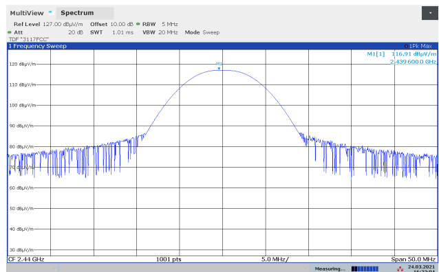
Maximum Field Strength, 2440 MHz, PLev 220, External Whip Ant
