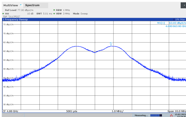
Emissions 4880 MHz, 2440 MHz, GFSK, VP, M70XC Ant
