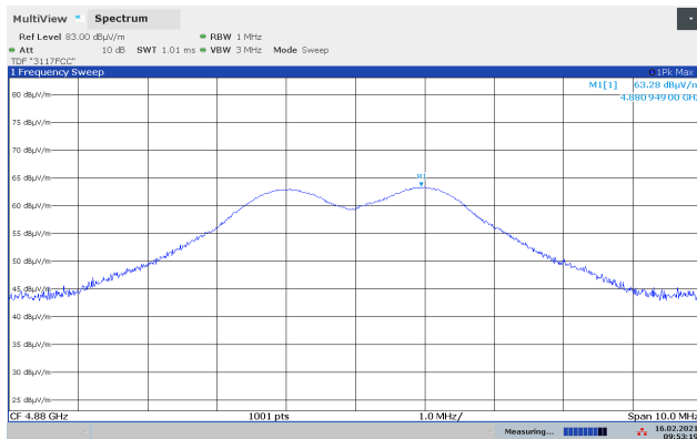
Emissions 4880 MHz, 2440 MHz, GFSK, VP, Int F-Ant
