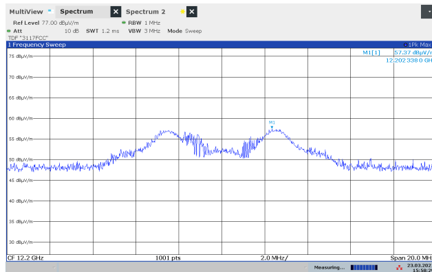
Emissions 12200 MHz, 2440 MHz, GFSK, VP, Ext Short Whip Ant
