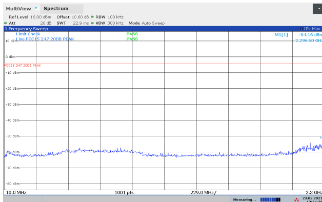
Conducted Emissions 10-2300 MHz, 2440 MHz, PLev 236
