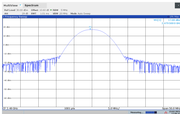
Peak Power, 2480 MHz, PLev 236
