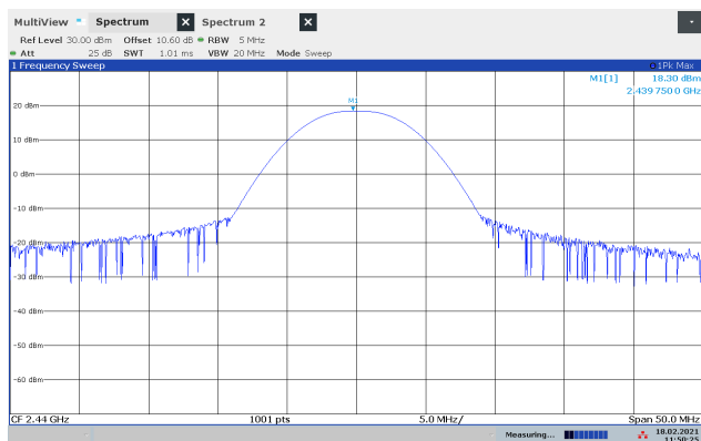
Peak Power, 2440 MHz, PLev 220
