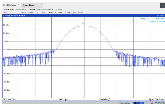
Peak Power, 2440 MHz, PLev 236
