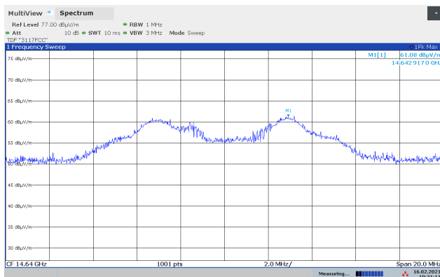
Emissions 14640 MHz, 2440 MHz, GFSK, VP, Int F-Ant
