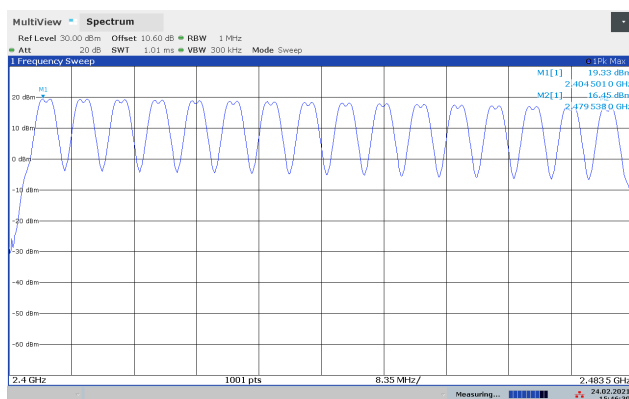
RF Channels in Use, Basic Rate
