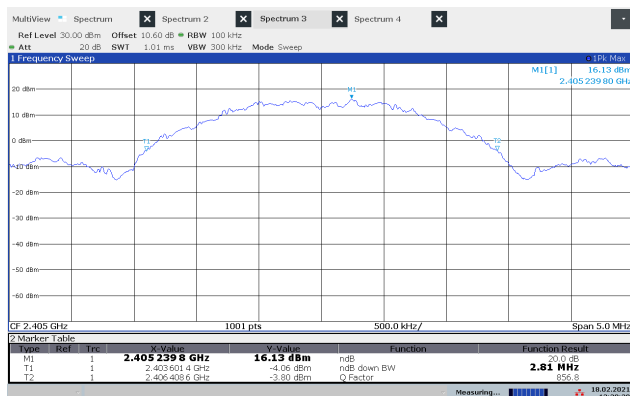
20dB Bandwidth 2405 MHz
