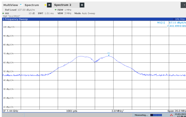
Emissions 7440 MHz, 2480 MHz, GFSK, VP, Int F-Ant
