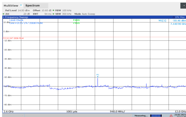
Conducted Emissions 2600-12000 MHz, 2480 MHz, PLev 236
