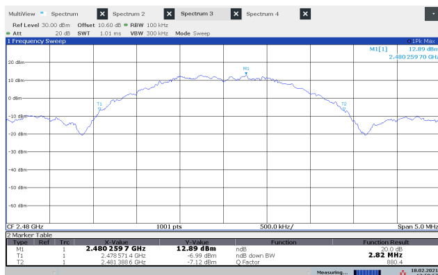
20dB Bandwidth 2480 MHz
