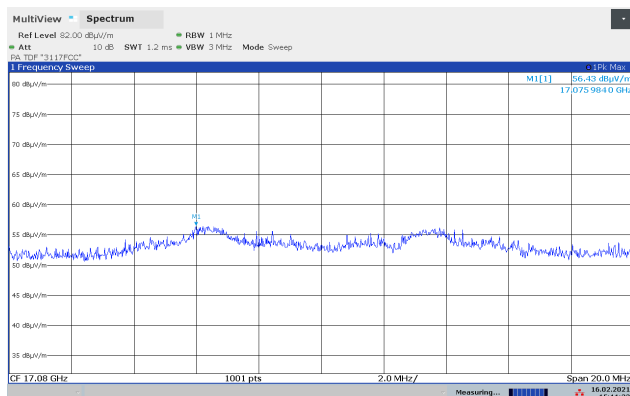
Emissions 17080 MHz, 2440 MHz, GFSK, HP, M70XC Ant
