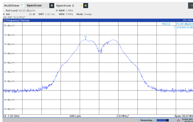
Emissions 7320 MHz, 2440 MHz, GFSK, VP, Ext Short Whip Ant
