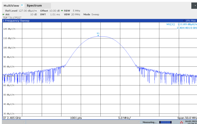
Maximum Field Strength, 2405 MHz, PLev 220, M70XC
