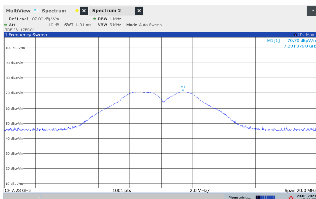
Emissions 7230 MHz, 2410 MHz, GFSK, VP, Int F-Ant
