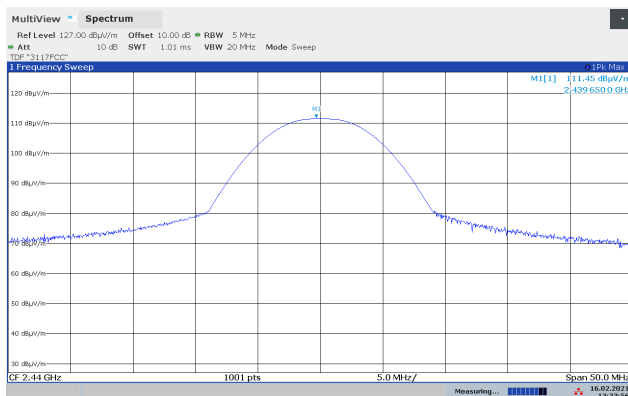
Maximum Field Strength, 2440 MHz, PLev 220, M70XC
