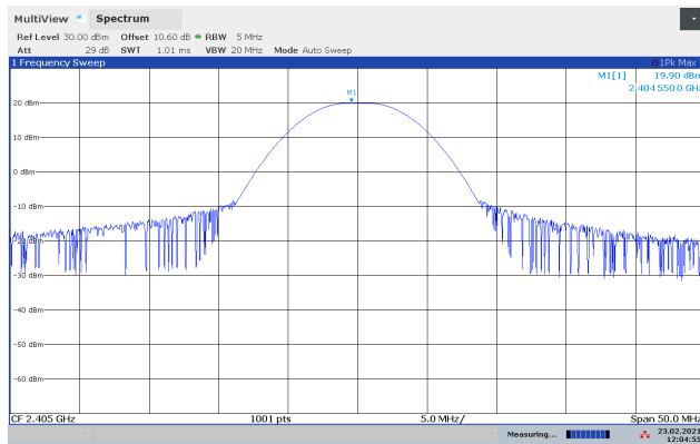
Peak Power, 2405 MHz, PLev 236
