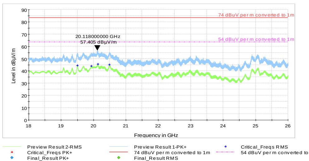
Plot #8 Radiated Emissions: 18 GHz - 26 GHz
