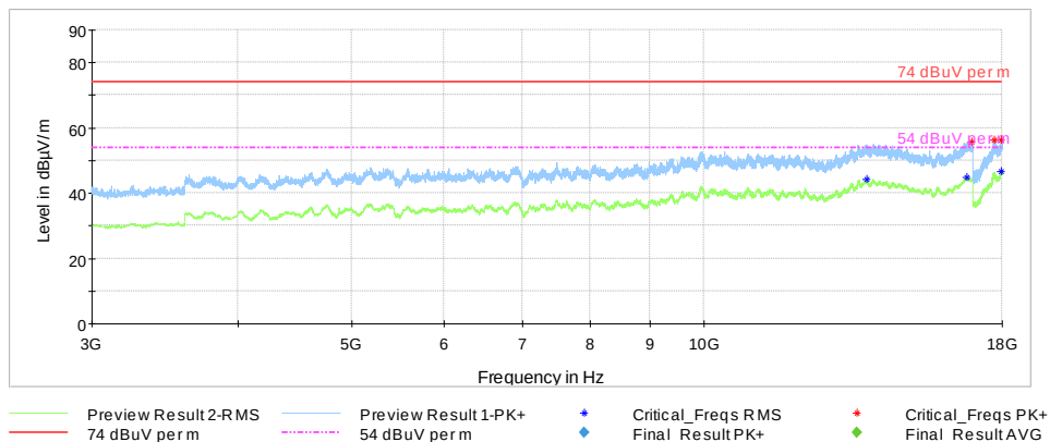
Plot #11 Radiated Emissions: 3 GHz -18 GHz
