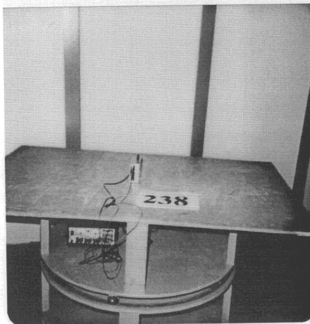
Radiated Emissions
