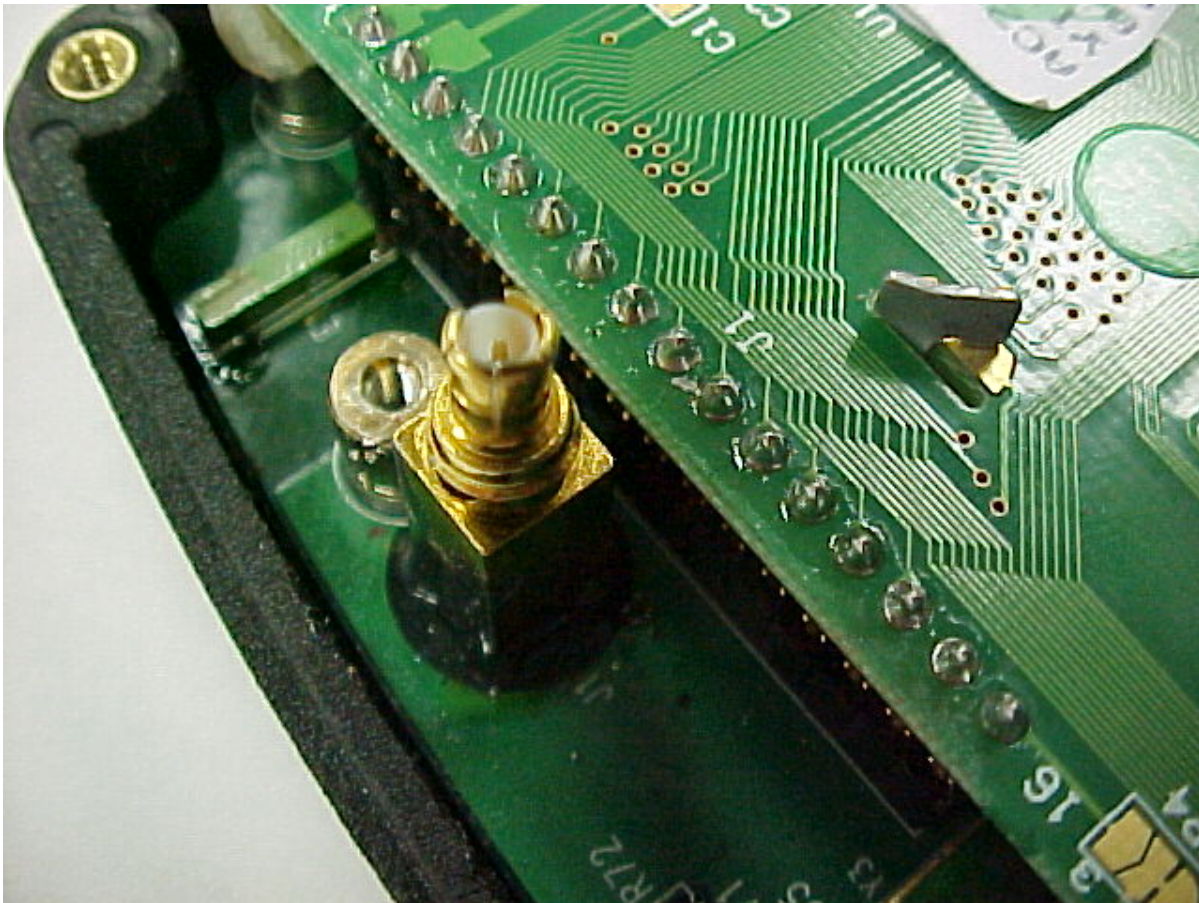
Photo Five – Internal Close Up of Antenna
