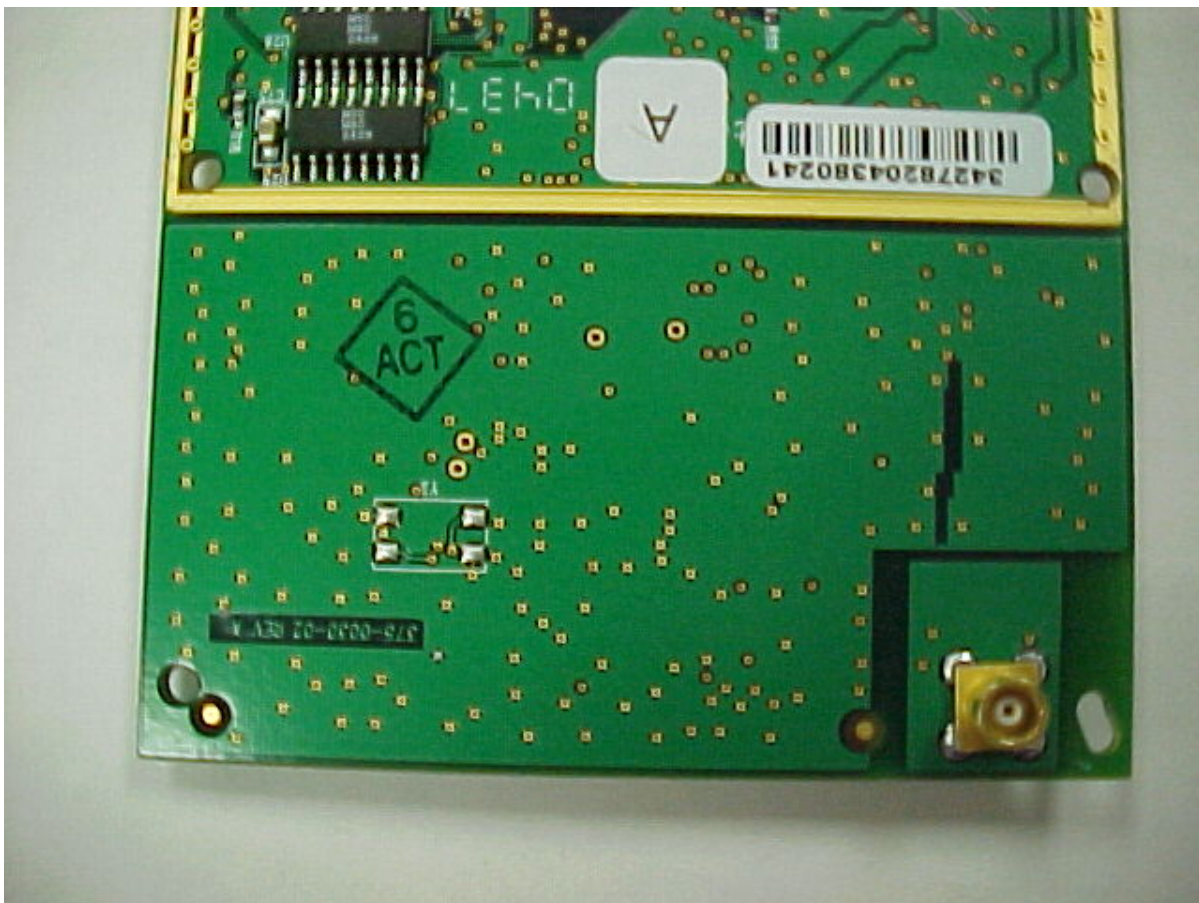
Photo Three – Internal RF Section, Non-Component Side
