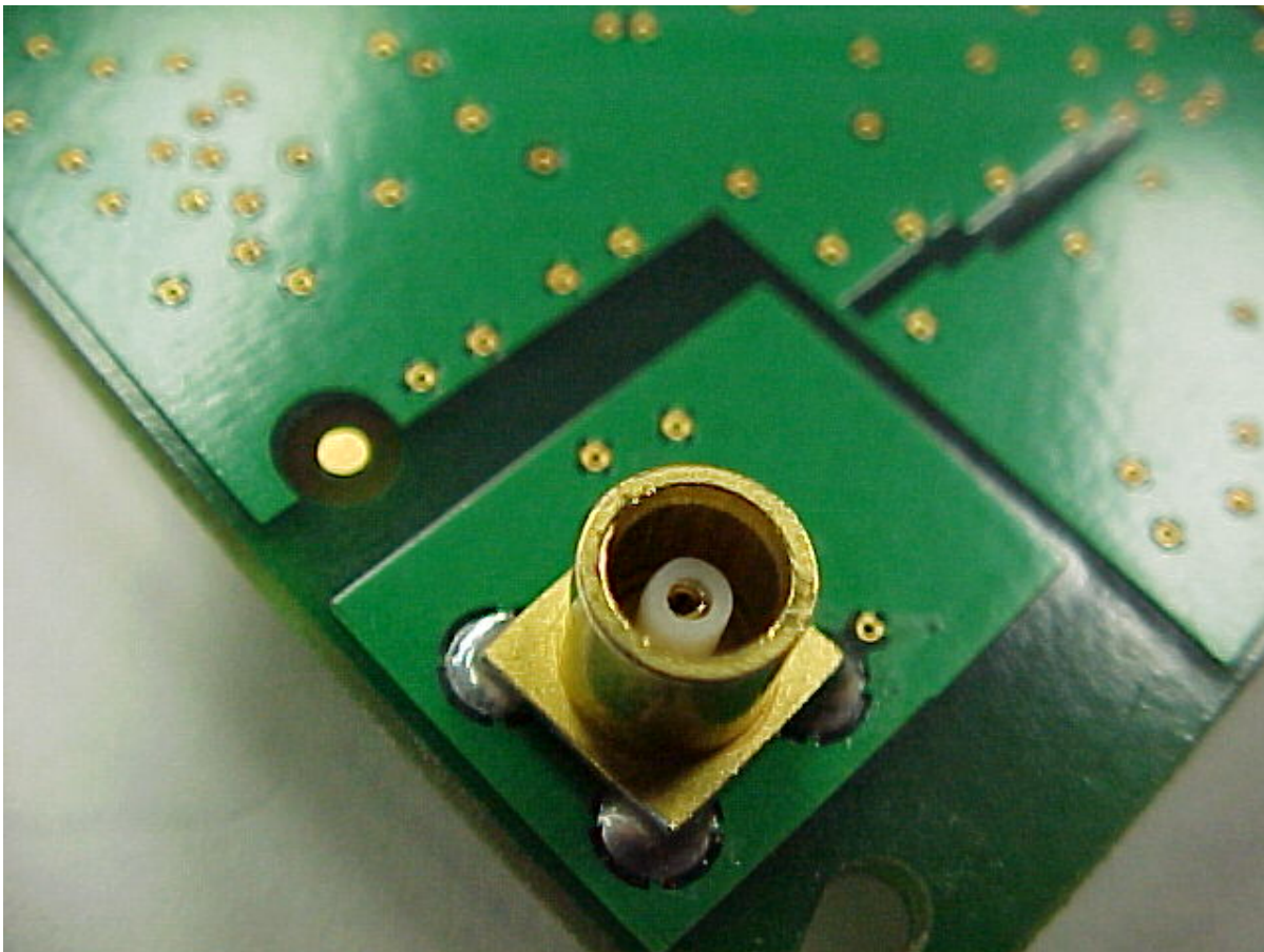
Photo Four – Internal Close Up of Antenna Connector
