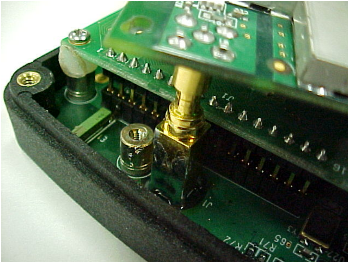
Photo Six – Internal Close Up of Antenna Port
