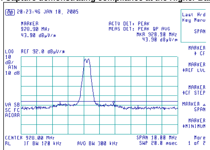
Screen Capture demonstrating compliance at the Higher Band-Edge
