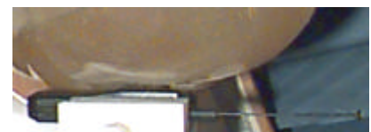
Fig. 14 Head SAR Test Setup
