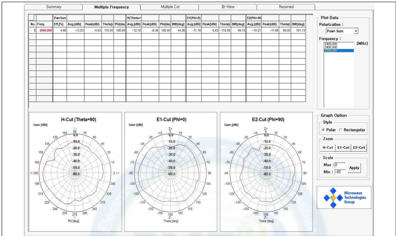
WAVE-P1_2.5GHz
