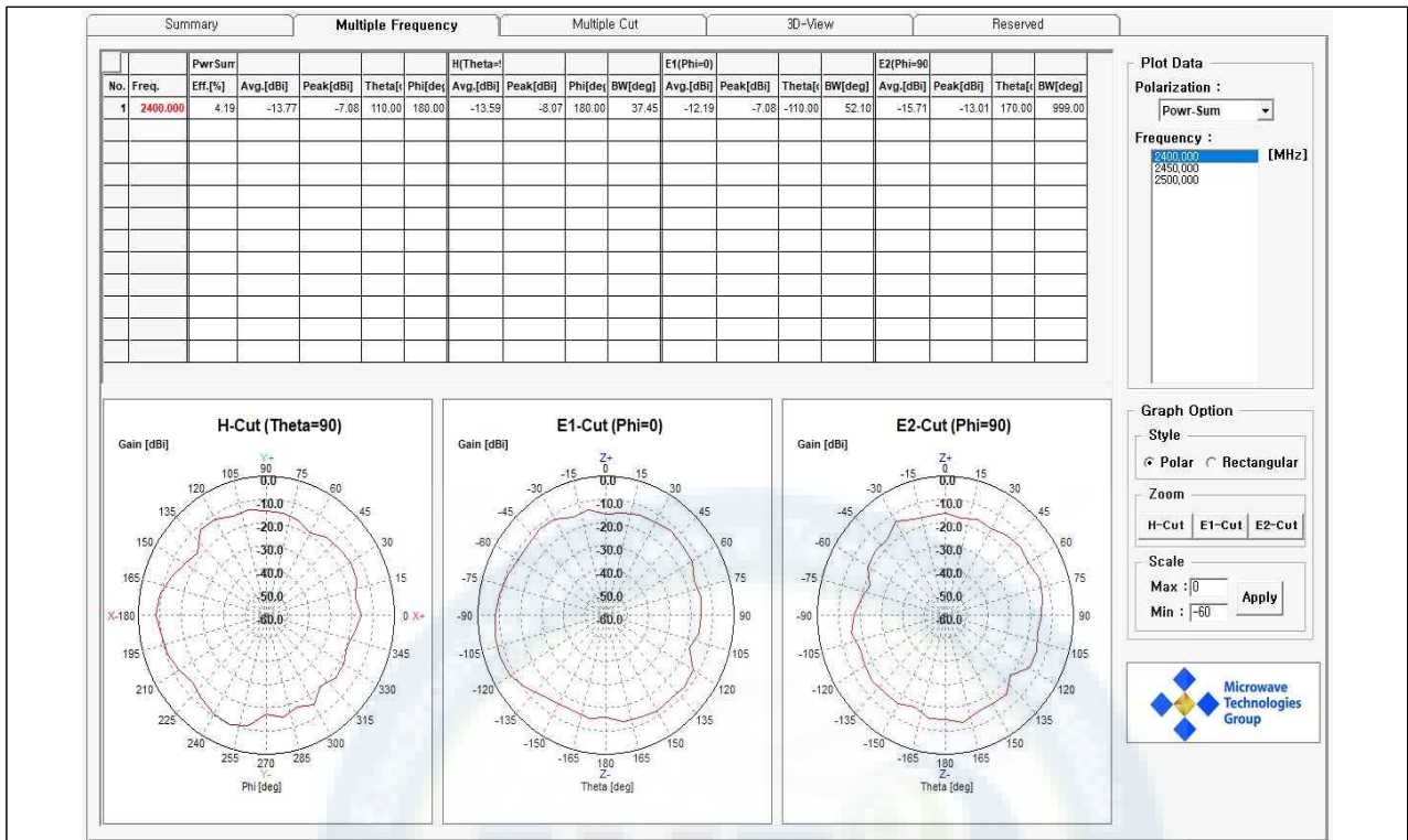
WAVE-P1_2.4GHz
