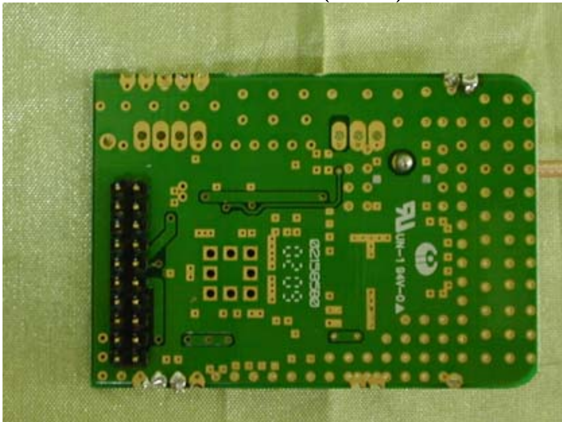
Internal Photo of EUT (Base Unit)
