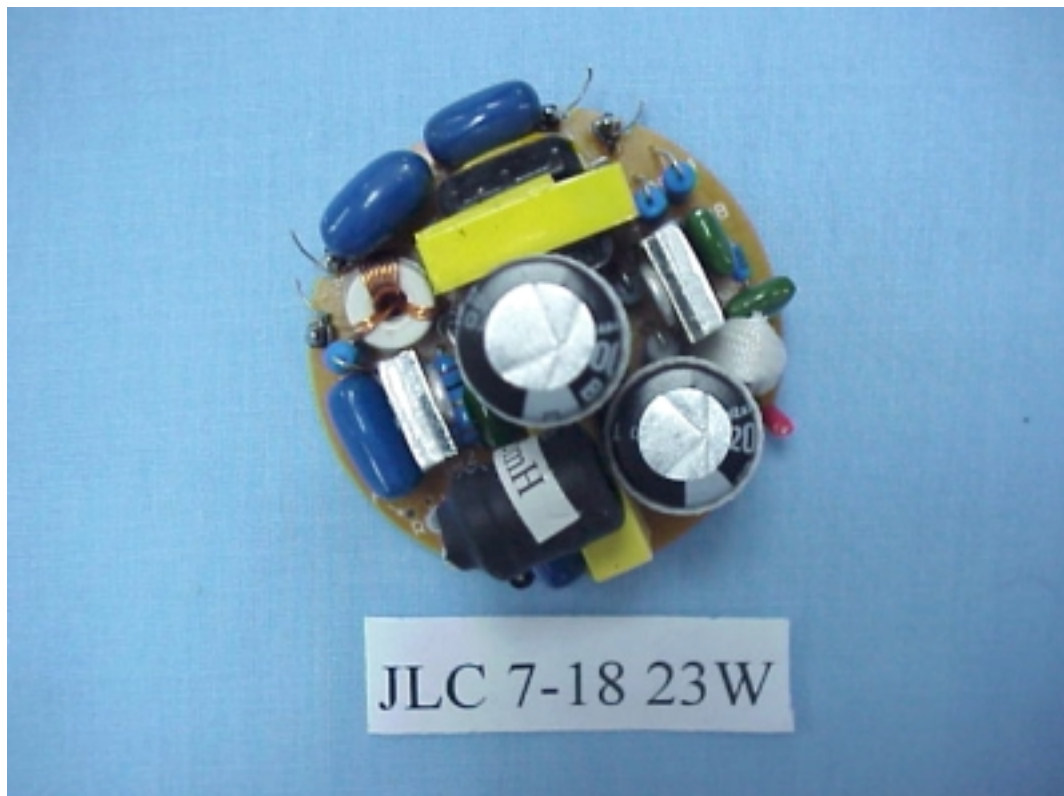
Figure 8 ENERGY SAVING LAMP (M/N: JLC 7-18 23W) Main Board (Component Side)
