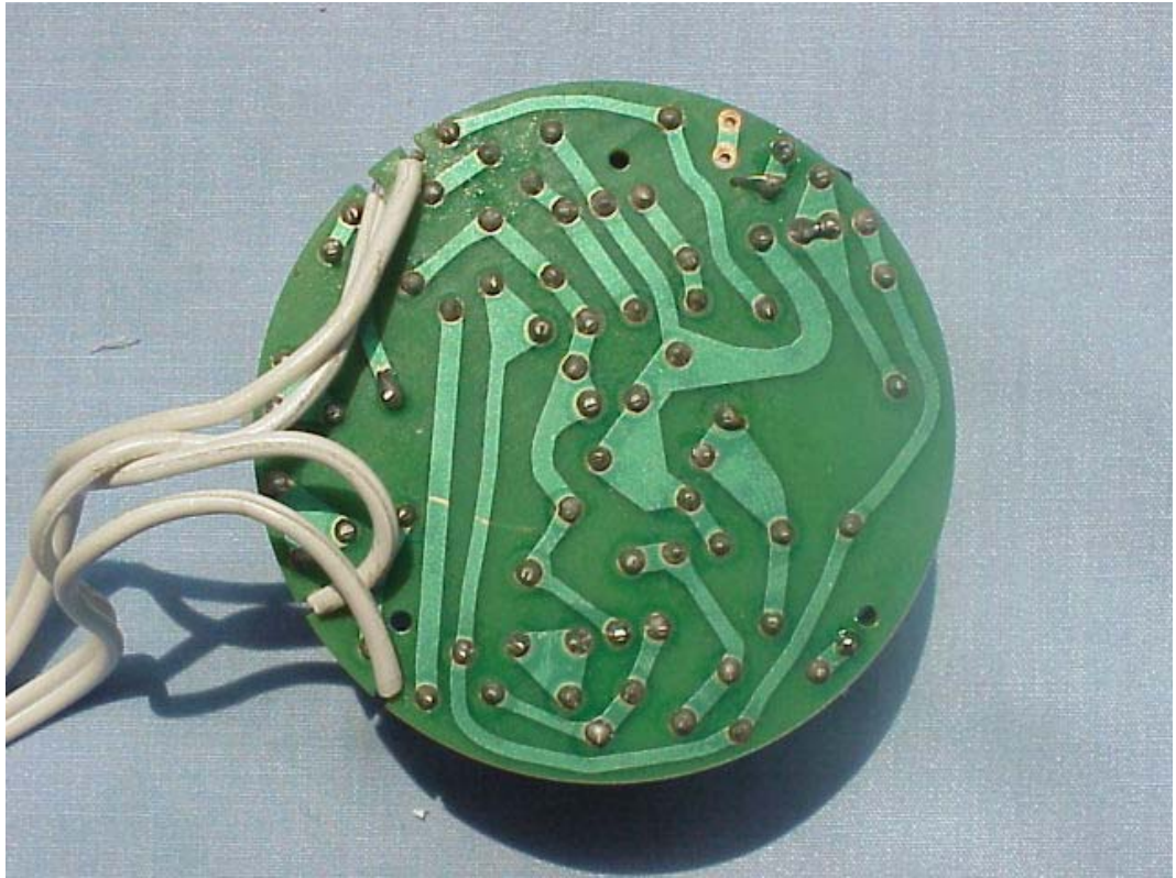
FIGURE 3 CIRCLINE LAMP (M/N: CIRCLINE 22W) MAIN BOARD (SOLDERED SIDE)
