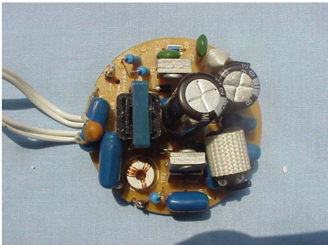
FIGURE 2 CIRCLINE LAMP (M/N: CIRCLINE 22W) MAIN BOARD (COMPONENT SIDE)
