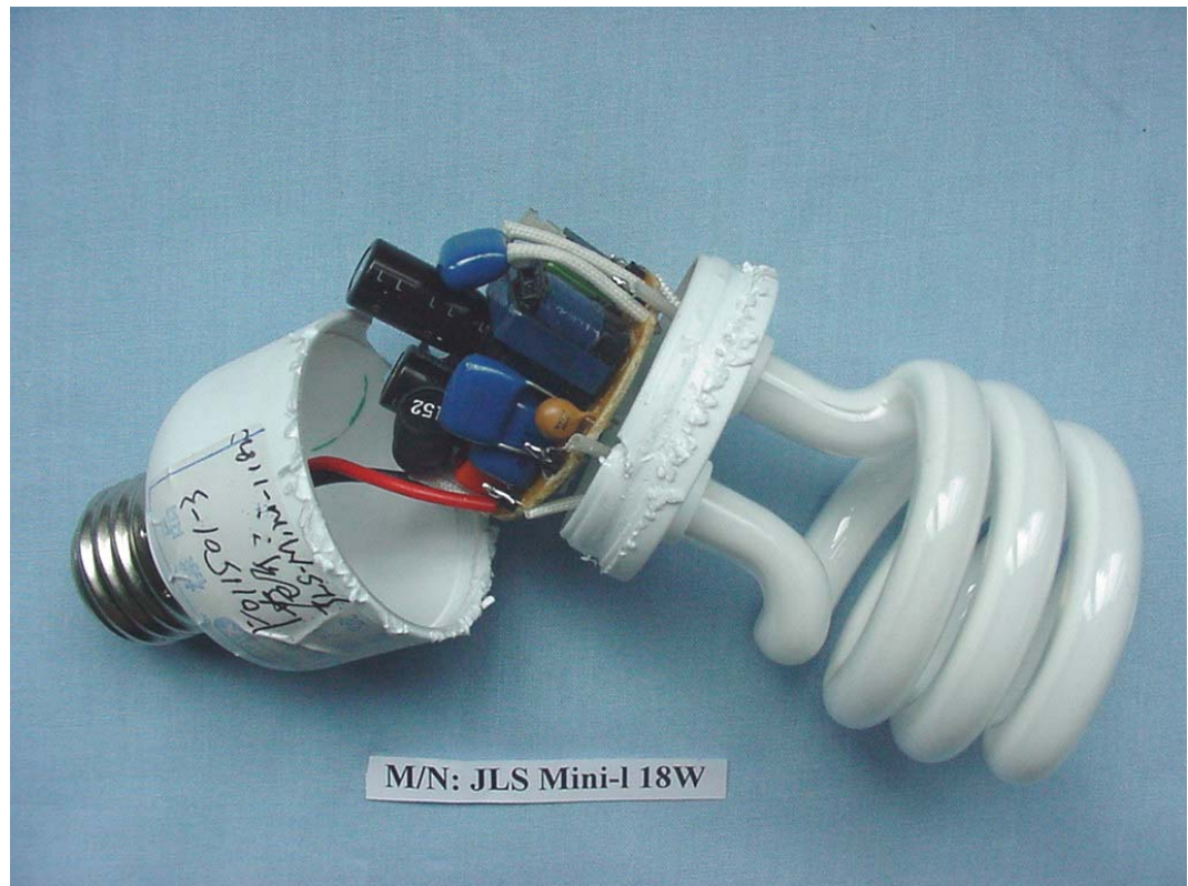
FIGURE 1 ENERGY SAVING LAMP (M/N: JLS MINI-I 18W) COVER REMOVED
