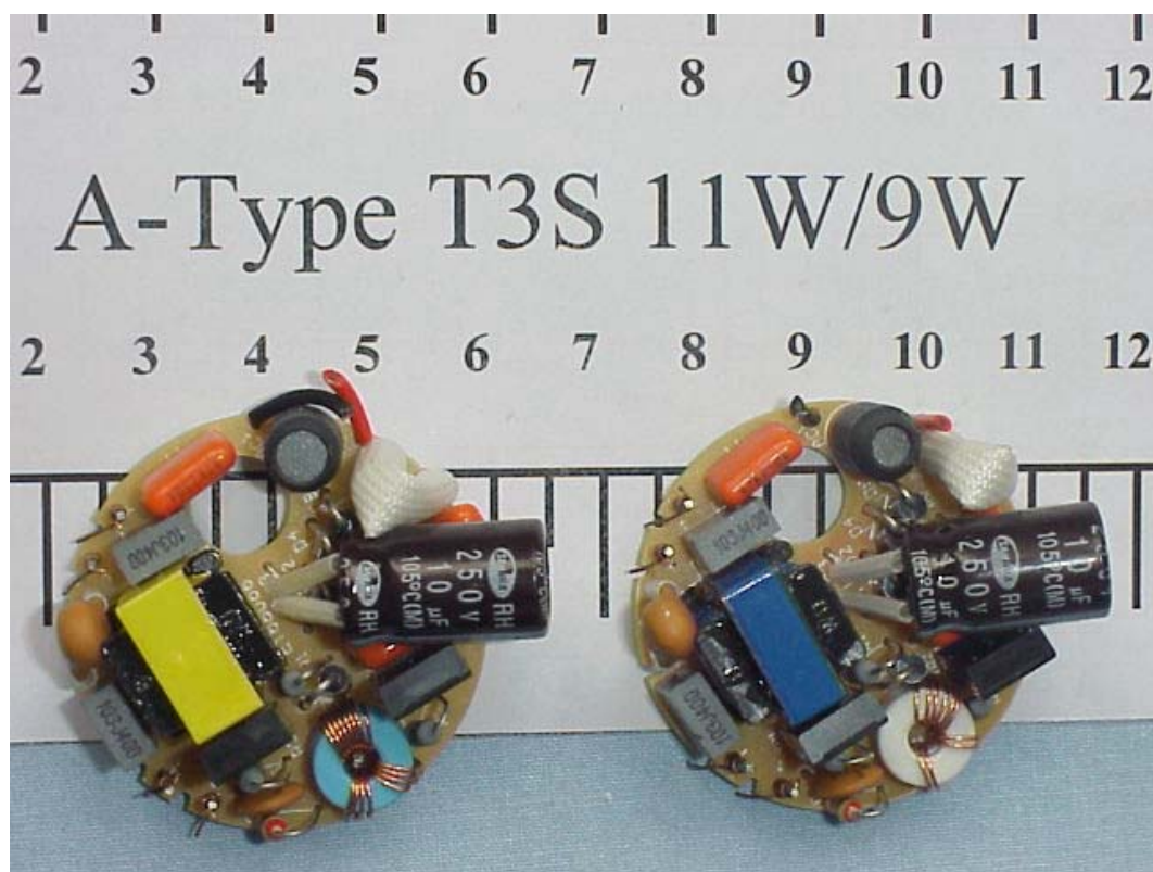
FIGURE 5 ENERGY SAVING LAMP (M/N: A-TYPE T3S 11W/9W) MAIN BOARD (COMPONENT SIDE)
