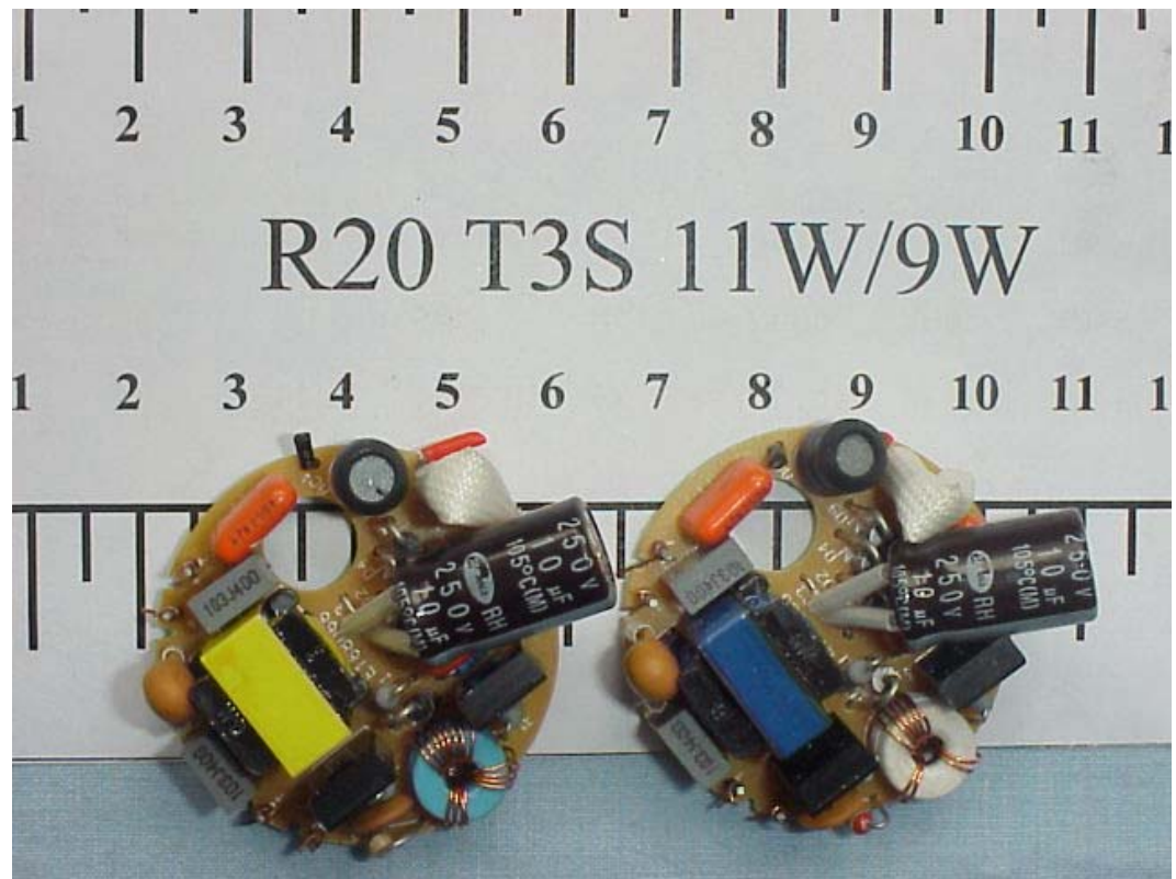
FIGURE 8 ENERGY SAVING LAMP (M/N: R20 T3S 11W/9W) MAIN BOARD (COMPONENT SIDE)
