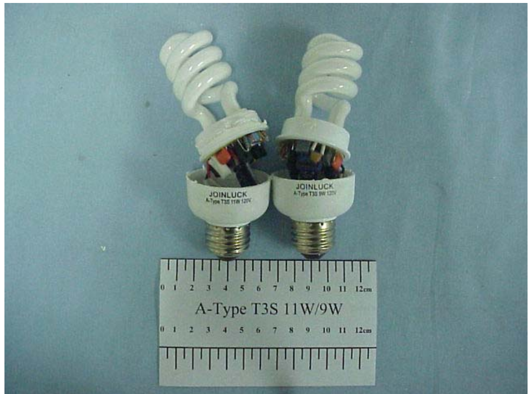
FIGURE 4 ENERGY SAVING LAMP (M/N: A-TYPE T3S 11W/9W) COVER REMOVED
