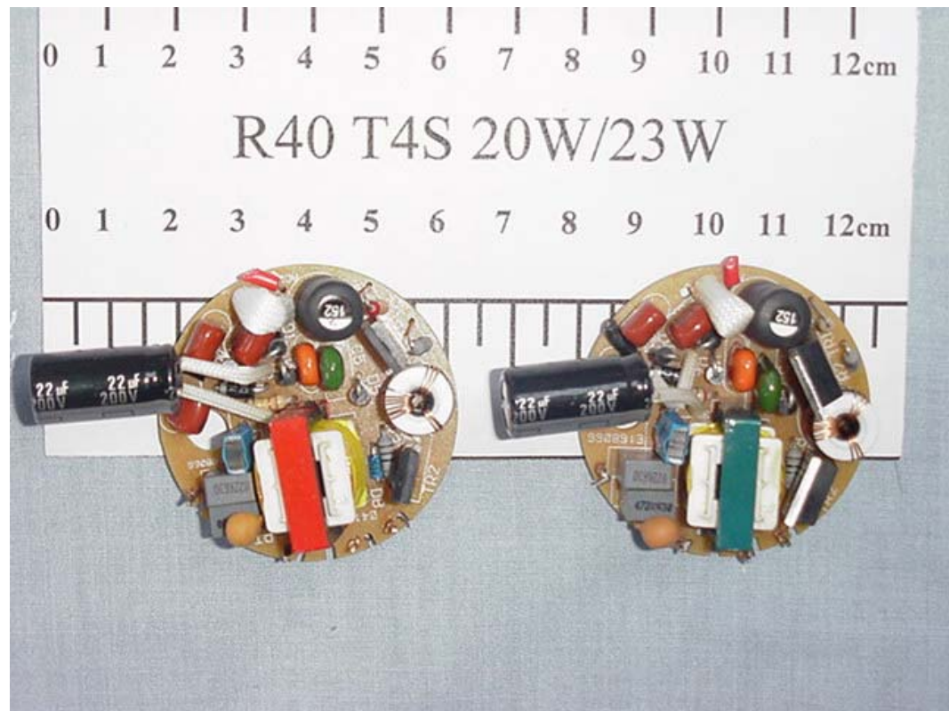
FIGURE 5 ENERGY SAVING LAMP (M/N: M/N: R40 T4S 20W/23W) MAIN BOARD (COMPONENT SIDE)
