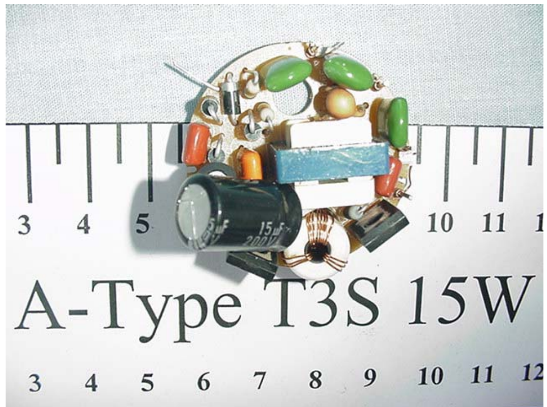
FIGURE 5 ENERGY SAVING LAMP (M/N: A-TYPE T3S 15W) MAIN BOARD (COMPONENT SIDE)
