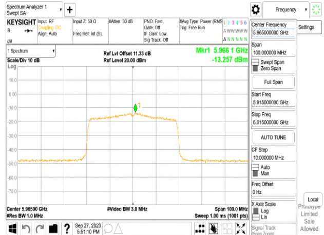
802.11ax_40MHz_Chain0_5965MHz_RU242_61
