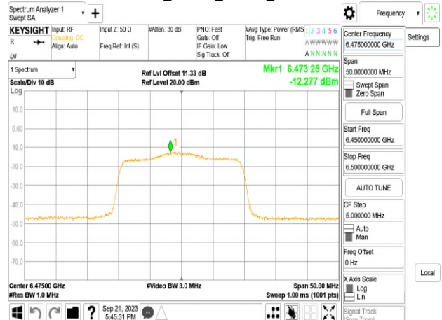
802.11a_20MHz_Chain1_6475MHz
