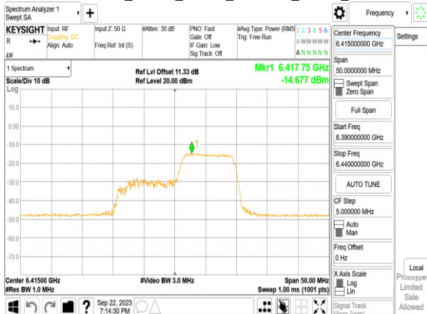
802.11ax_20MHz_Chain0_6415MHz_RU106_54
