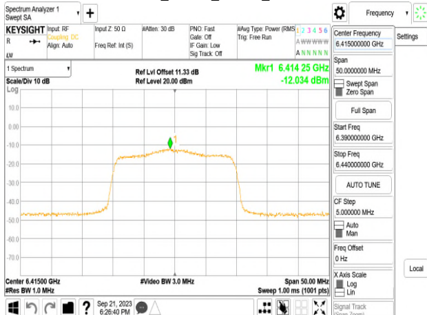
802.11ax_20MHz_Chain1_6415MHz
