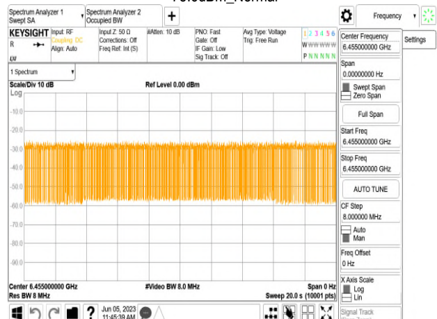
802.11ax_20MHz_CF 6455MHz_Interference_6455MHz_ -75.6dBm_Normal
