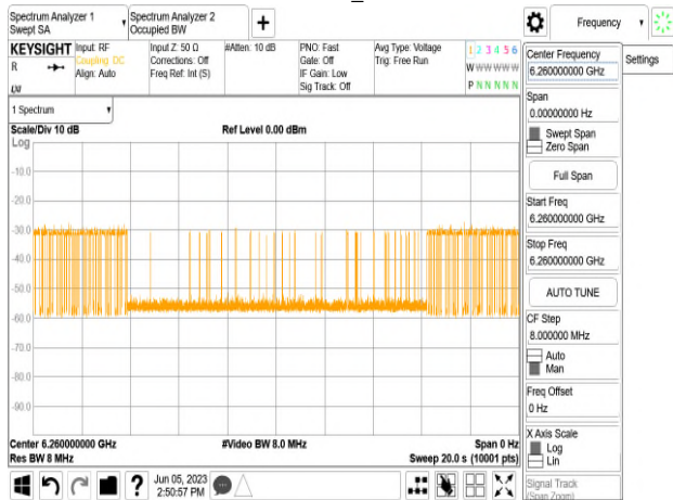
802.11ax_160MHz_CF 6185MHz_Interference_6260MHz_ -78.53dBm_Normal
