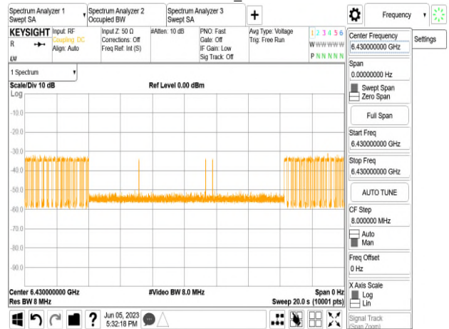
802.11ax_160MHz_CF 6505MHz_Interference_6430MHz_ -74.59dBm_Normal
