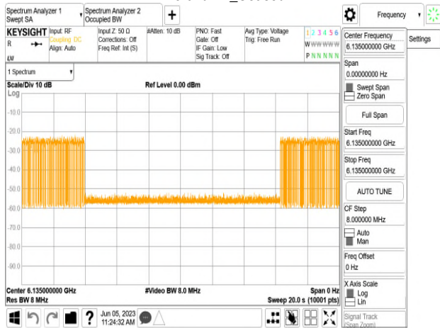
802.11ax_20MHz_CF 6135MHz_Interference_6135MHz_ -76.64dBm_Minimal
