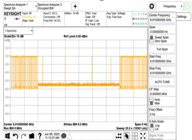
802.11ax_160MHz_CF 6985MHz_Interference_6910MHz_ -76.28dBm_Normal
