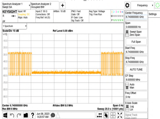
802.11ax_160MHz_CF 6665MHz_Interference_6740MHz_ -76.26dBm_Minimal
