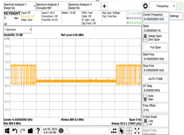
802.11ax_160MHz_CF 6505MHz_Interference_6430MHz_ -73.59dBm_Minimal
