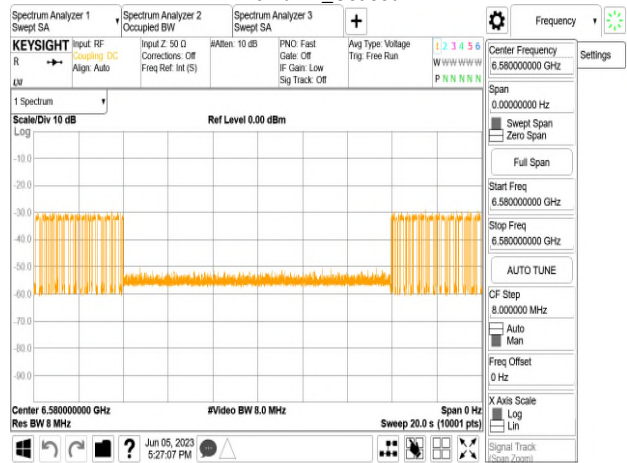
802.11ax_160MHz_CF 6505MHz_Interference_6580MHz_-74.7dBm_Minimal
