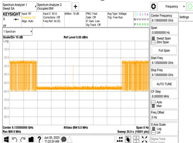
802.11ax_20MHz_CF 6135MHz_Interference_6135MHz_ -78.64dBm_Normal
