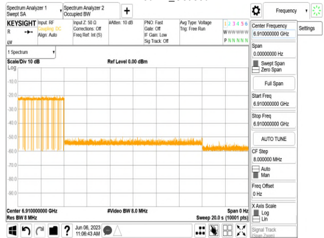
802.11ax_160MHz_CF 6985MHz_Interference_6910MHz_ -73.28dBm_Minimal
