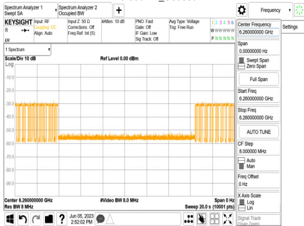
802.11ax_160MHz_CF 6185MHz_Interference_6260MHz_ -76.53dBm_Minimal
