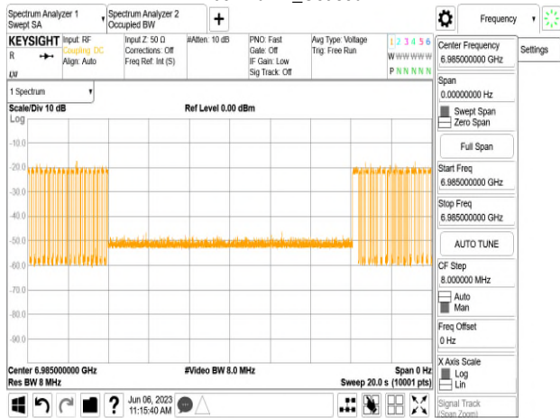
802.11ax_160MHz_CF 6985MHz_Interference_6985MHz_-69.22dBm_Minimal
