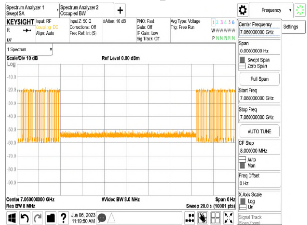
802.11ax_160MHz_CF 6985MHz_Interference_7060MHz_-73.29dBm_Minimal
