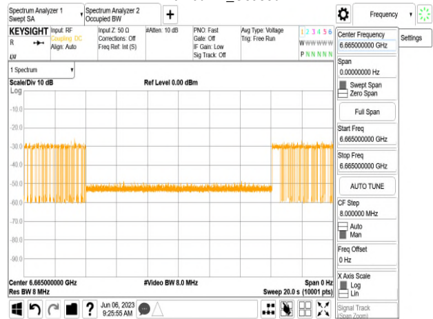
802.11ax_160MHz_CF 6665MHz_Interference_6665MHz_-71.16dBm_Minimal
