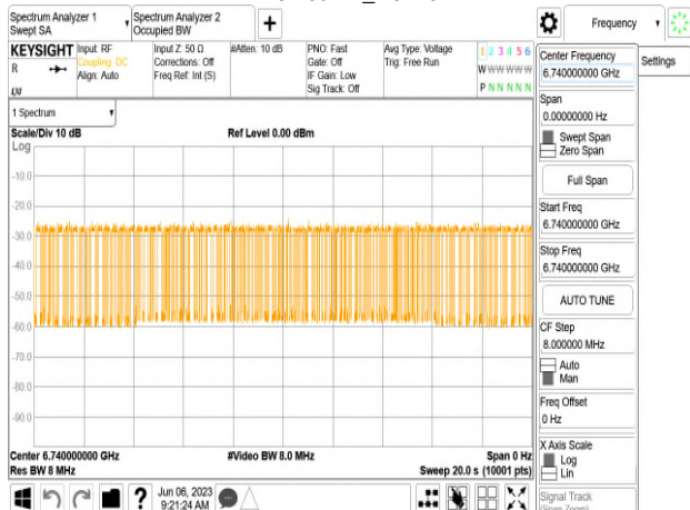
802.11ax_160MHz_CF 6665MHz_Interference_6740MHz_ -78.26dBm_Normal
