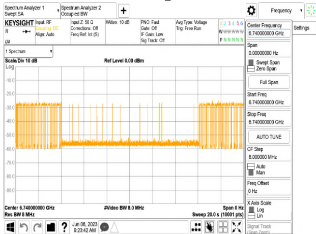
802.11ax_160MHz_CF 6665MHz_Interference_6740MHz_ -78.26dBm_Normal
