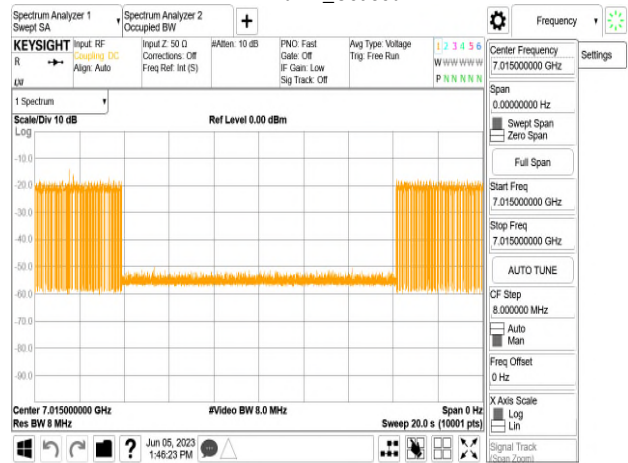
802.11ax_20MHz_CF 7015MHz_Interference_7015MHz_-75.2dBm_Minimal
