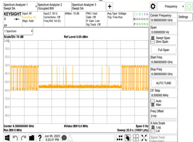
802.11ax_160MHz_CF 6505MHz_Interference_6580MHz_-77.7dBm_Normal
