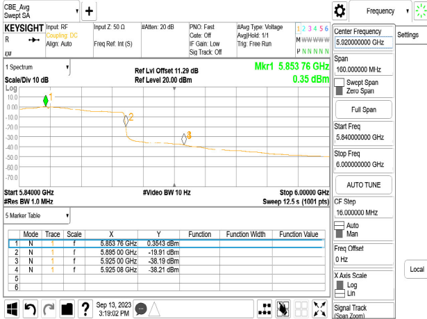
Chain1_5855_Avg
