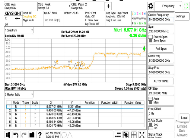
Chain0_5570_996_S67_Peak
