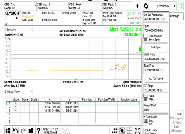
Chain0_5250_Peak-2
