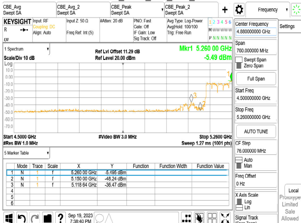
Chain0_5250_Avg-2
