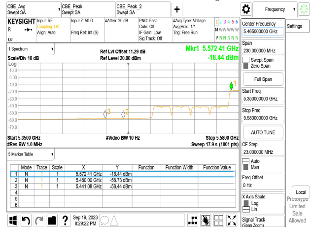
Chain0_5570_996_S67_Peak-2
