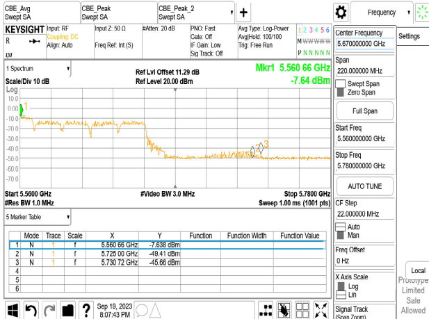
Chain0_5570_996_67_Peak
