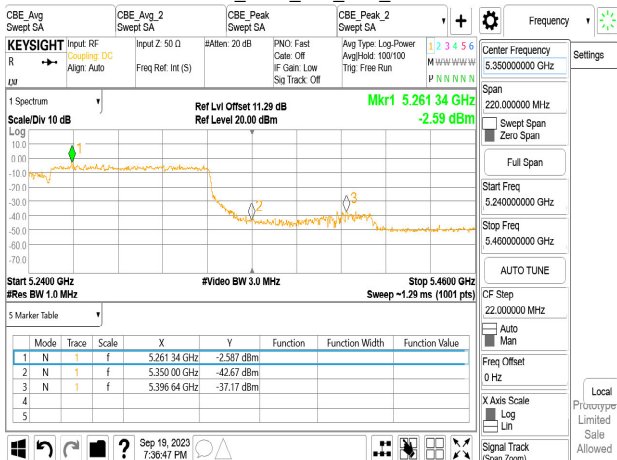
Chain0_5250_996_S67_Peak
