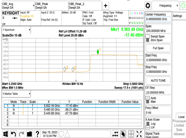
Chain0_5570_996_67_Peak-2
