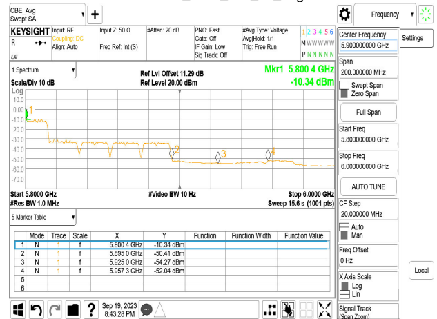
Chain1_5815_996_S67_Avg
