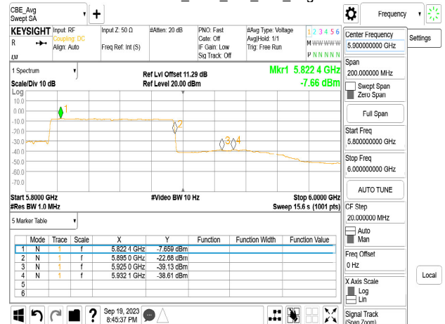
Chain1_5815_Avg
