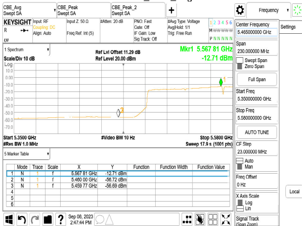
Chain1_5570_Peak-2
