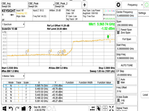
Chain1_5570_Peak
