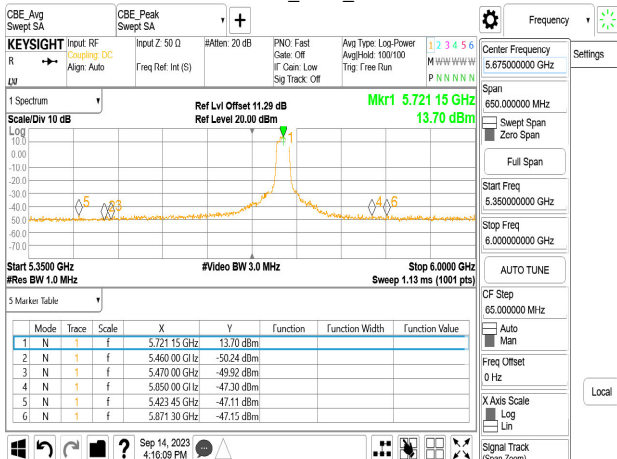
Chain1_5720_Peak
