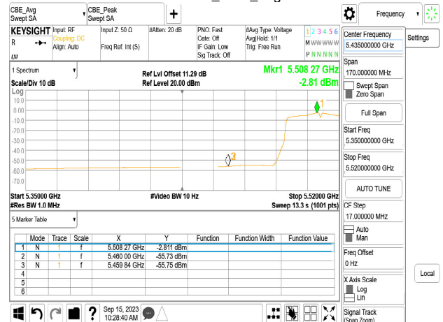
Chain1_5510_Peak
