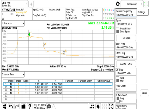
Chain1_5875_Avg
