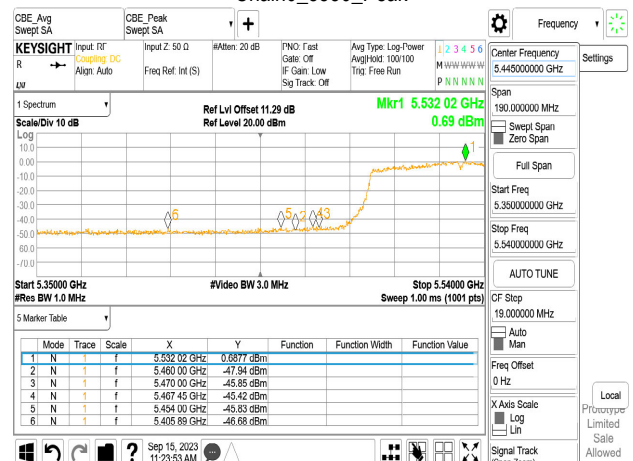
Chain0_5530_Peak
