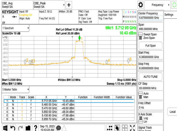
Chain1_5710_Peak
