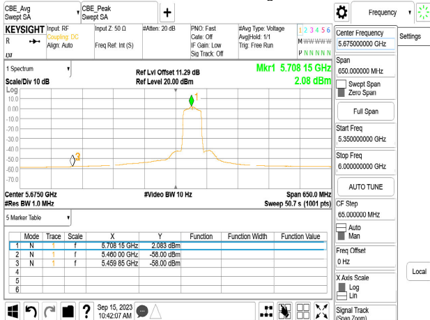
Chain1_5710_Peak
