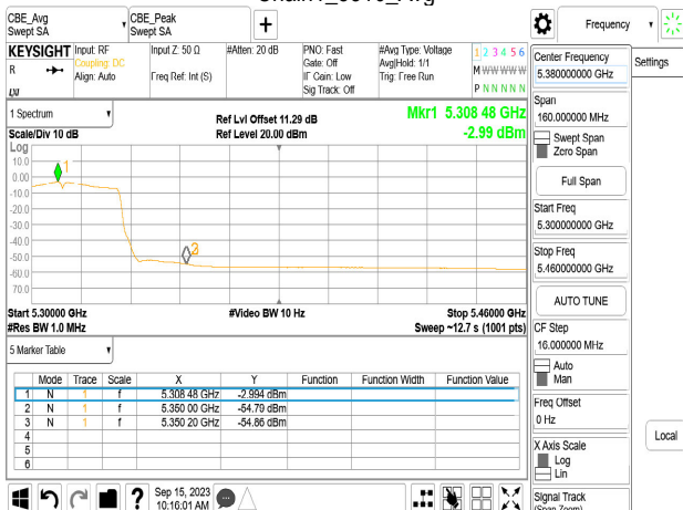
Chain1_5310_Avg
