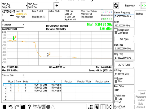
Chain0_5290_Avg
