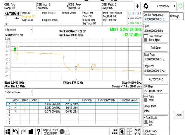
Chain1_5250_Peak_L
