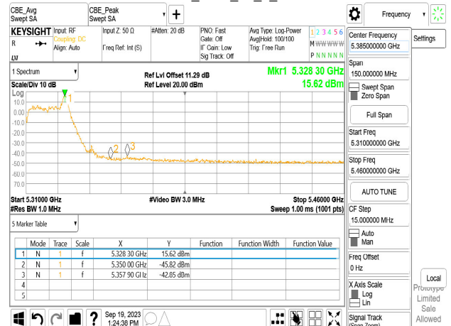
Chain0_5320_26_8_Peak
