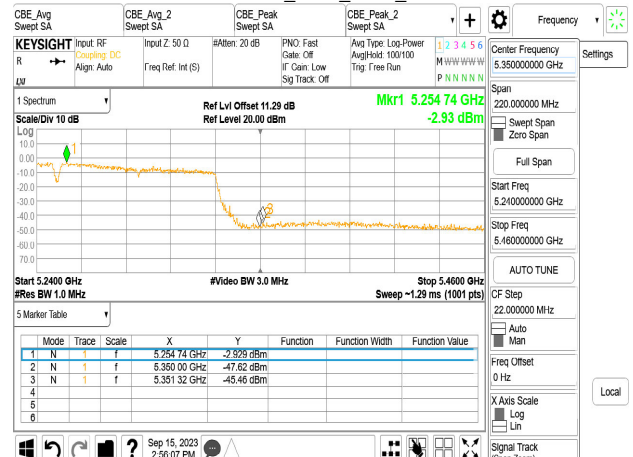
Chain1_5250_Peak_R
