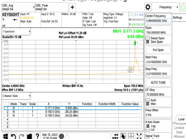
Chain0_5180_26_0_Avg
