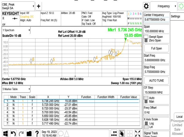
Chain0_5745_26_0_Peak
