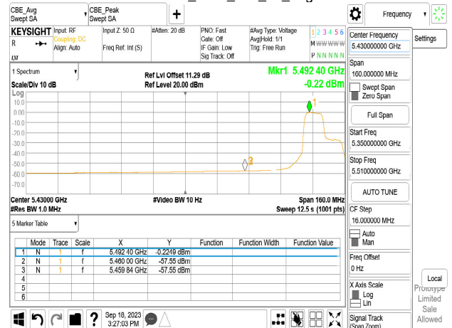
Chain0_5500_106_53_Peak
