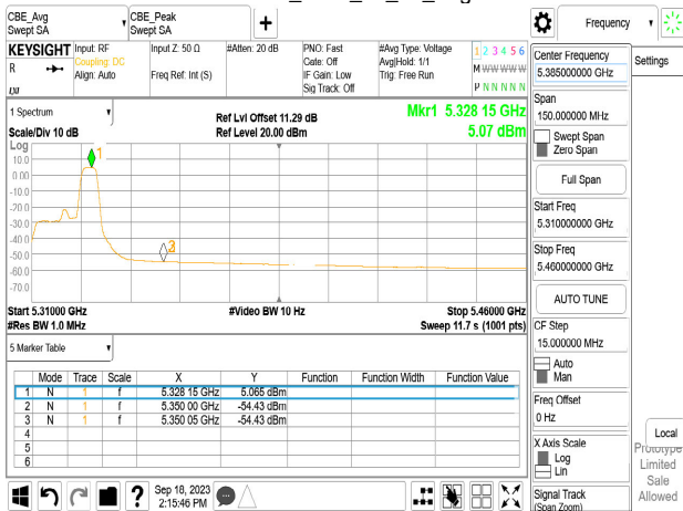
Chain0_5320_52_40_Peak
