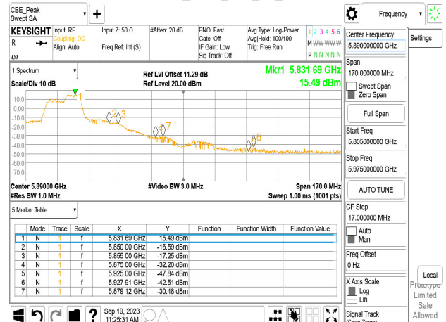
Chain0_5825_26_8_Peak
