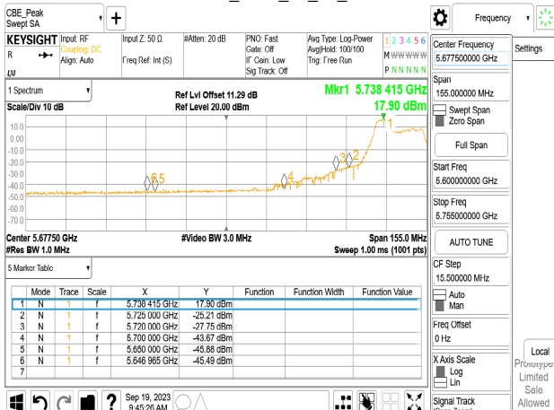
Chain0_5745_52_37_Peak
