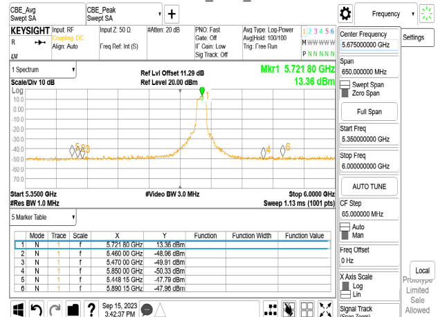
Chain0_5720_Peak
