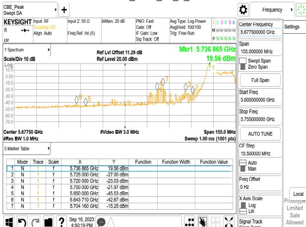
Chain0_5745_52_37_Peak
