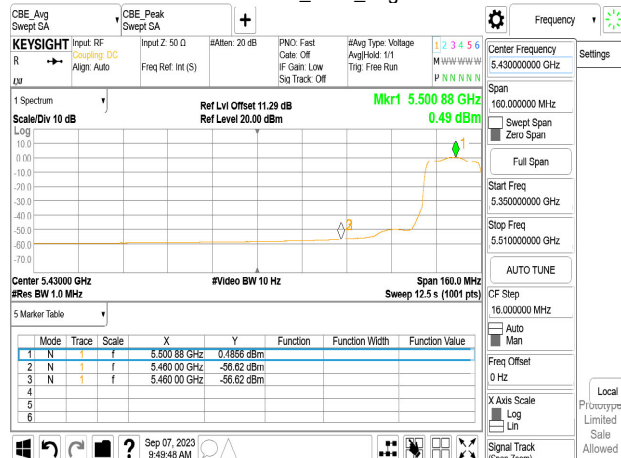
Chain0_5500_Peak
