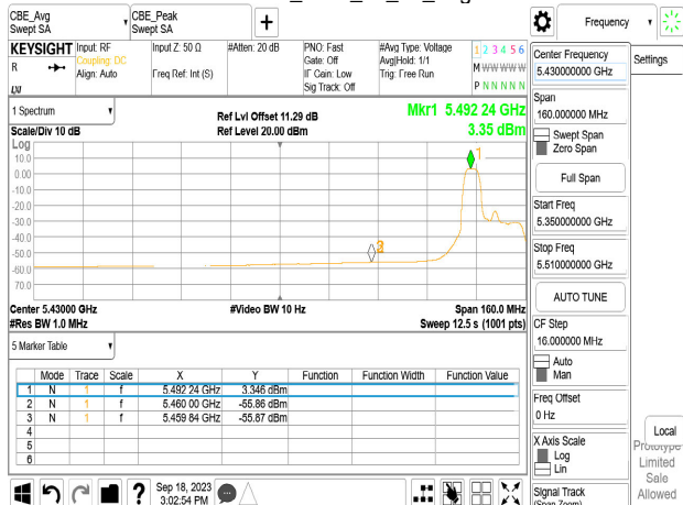
Chain0_5500_52_37_Avg
