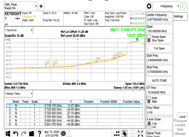
Chain0_5825_106_54_Peak
