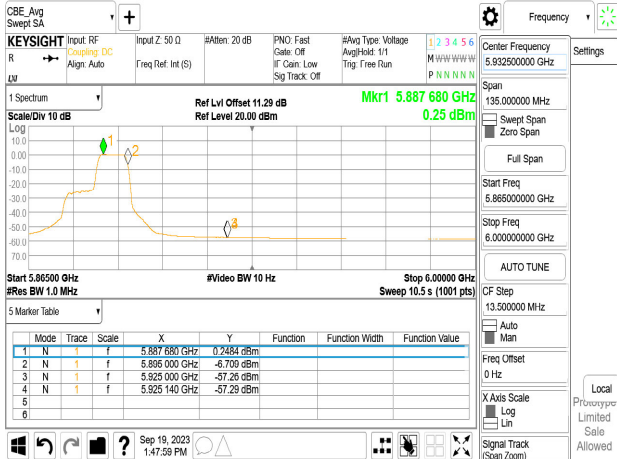
Chain0_5885_106_54_Avg
