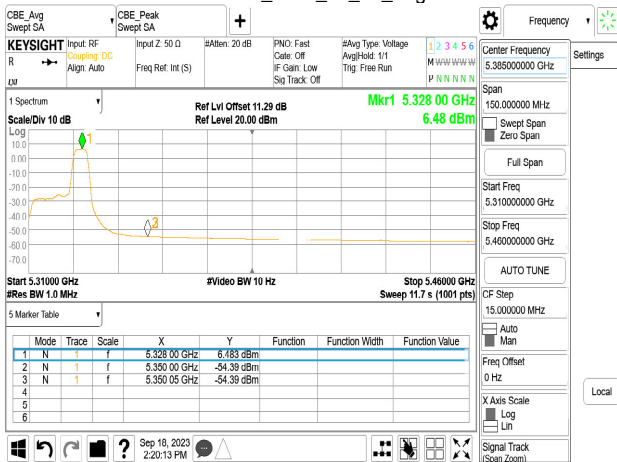
Chain1_5320_52_40_Peak
