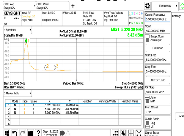
Chain1_5320_26_8_Peak
