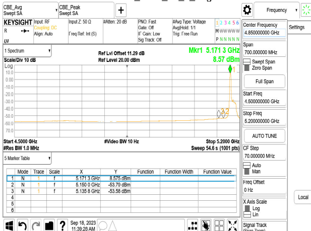
Chain1_5180_26_0_Avg
