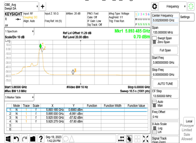
Chain0_5885_52_40_Avg
