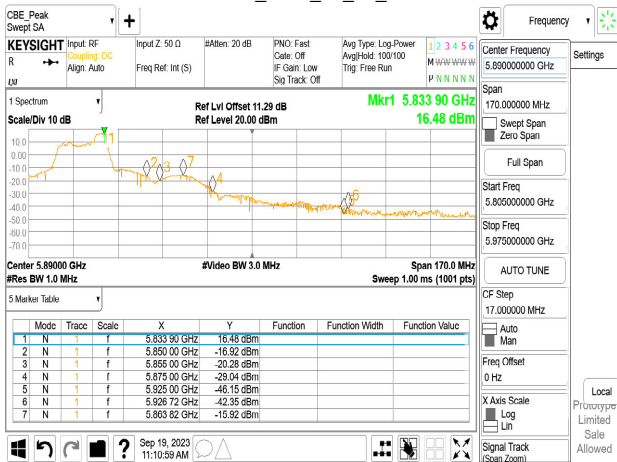
Chain0_5825_Peak
