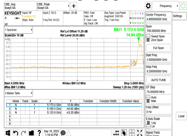
Chain1_5180_52_37_Peak
