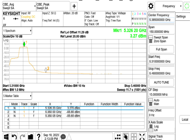
Chain1_5320_106_54_Avg
