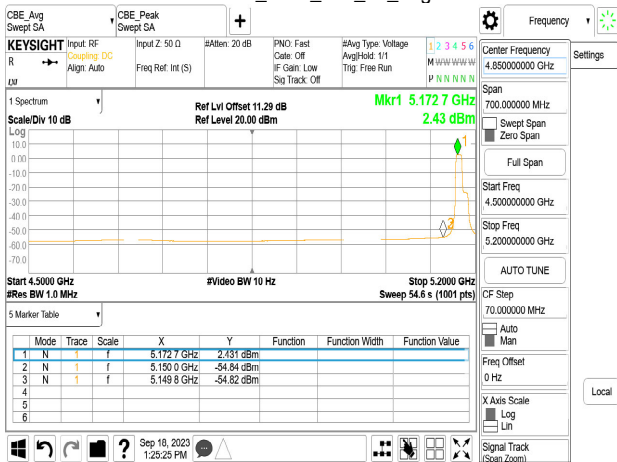
Chain1_5180_106_53_Peak
