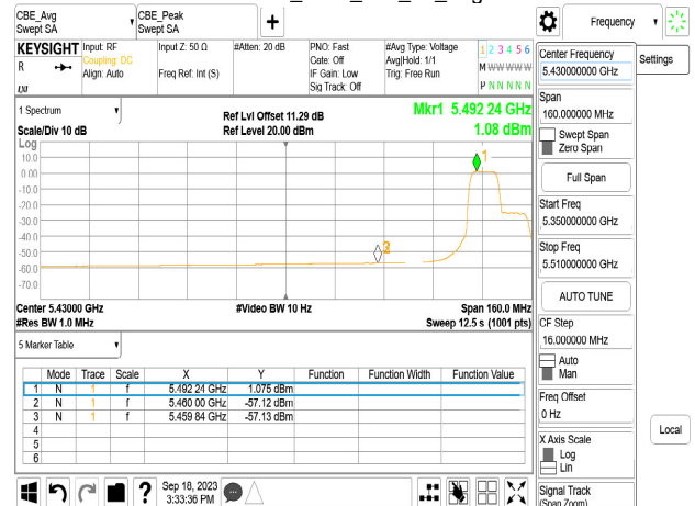
Chain1_5500_106_53_Peak
