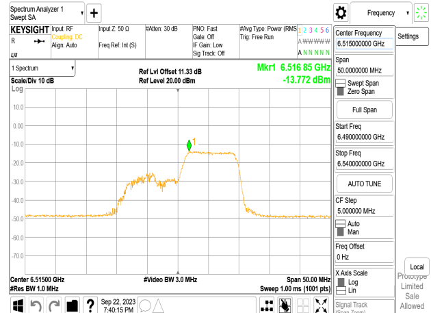
802.11ax_20MHz_Chain0_6515MHz_RU106_54
