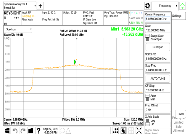
802.11ax_80MHz_Chain0_5985MHz_RU484_65
