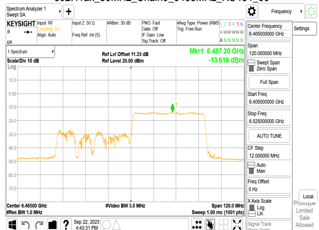
802.11ax_80MHz_Chain0_6465MHz_RU484_66
