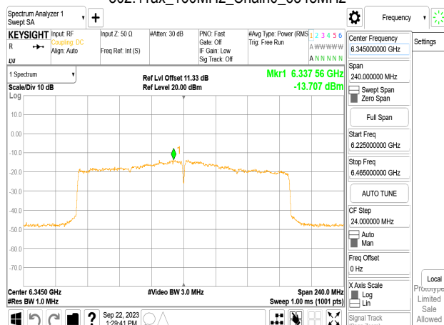
802.11ax_160MHz_Chain0_6345MHz_RU996_S67
