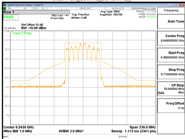
802.11ax_80MHz_6545MHz_V
