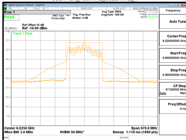
802.11ax_160MHz_6025MHz_V
