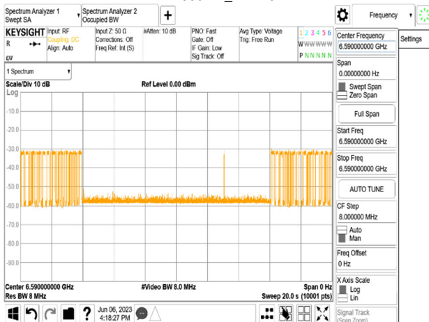
802.11ax_160MHz_CF 6665MHz_Interference_6590MHz_-75.99dBm_Normal
