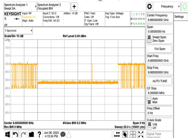
802.11ax_160MHz_CF 6665MHz_Interference_6665MHz_-70.72dBm_Normal
