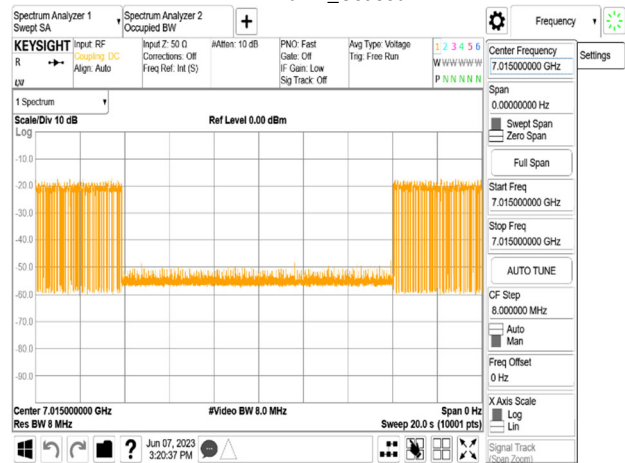
802.11ax_20MHz_CF 7015MHz_Interference_7015MHz_-73.77dBm_Minimal
