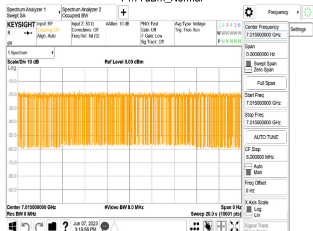
802.11ax_20MHz_CF 7015MHz_Interference_7015MHz_-74.77dBm_Normal
