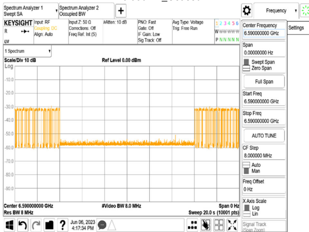
802.11ax_160MHz_CF 6665MHz_Interference_6590MHz_-72.99dBm_Minimal
