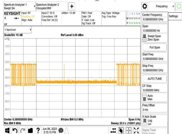
802.11ax_160MHz_CF 6505MHz_Interference_6580MHz_-72.57dBm_Normal
