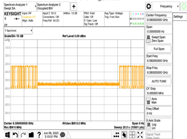
802.11ax_160MHz_CF 6505MHz_Interference_6580MHz_-71.57dBm_Minimal
