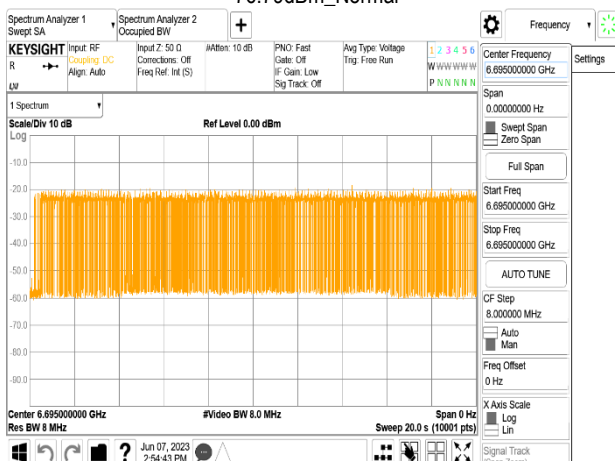
802.11ax_20MHz_CF 6695MHz_Interference_6695MHz_-76.79dBm_Normal
