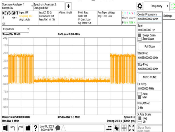
802.11ax_20MHz_CF 6695MHz_Interference_6695MHz_-75.79dBm_Minimal
