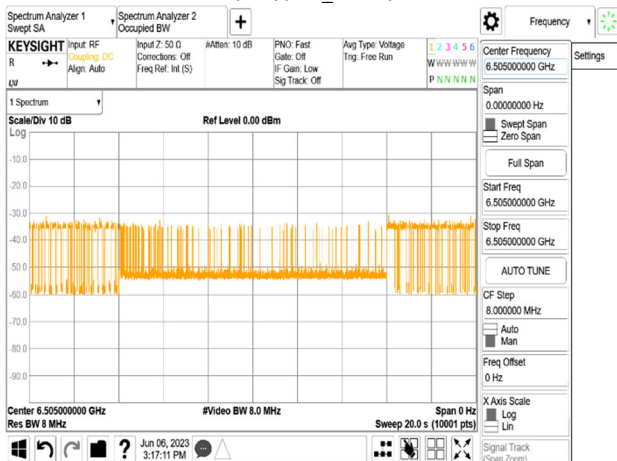
802.11ax_160MHz_CF 6505MHz_Interference_6505MHz_-69.46dBm_Normal
