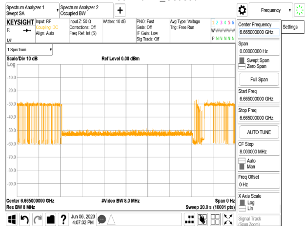
802.11ax_160MHz_CF 6665MHz_Interference_6665MHz_-68.72dBm_Minimal
