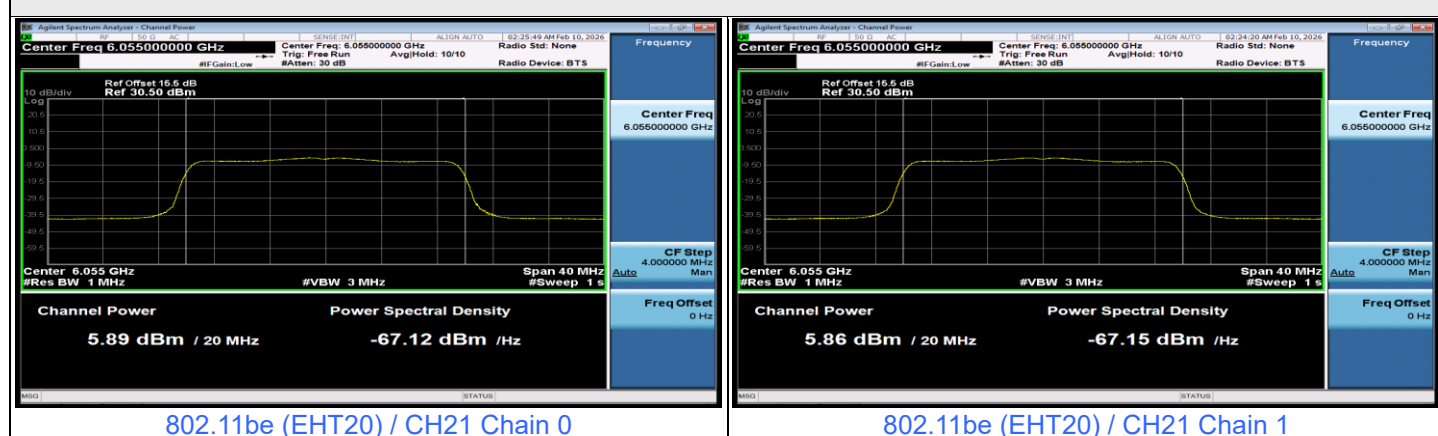
Client Plot of Power when associated with Low Power Indoor AP
