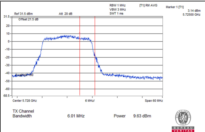
Chain 0 : CH 144 (U-NII-3)
