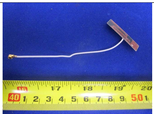
Ethertronics 1004078 Antenna – Bottom View
