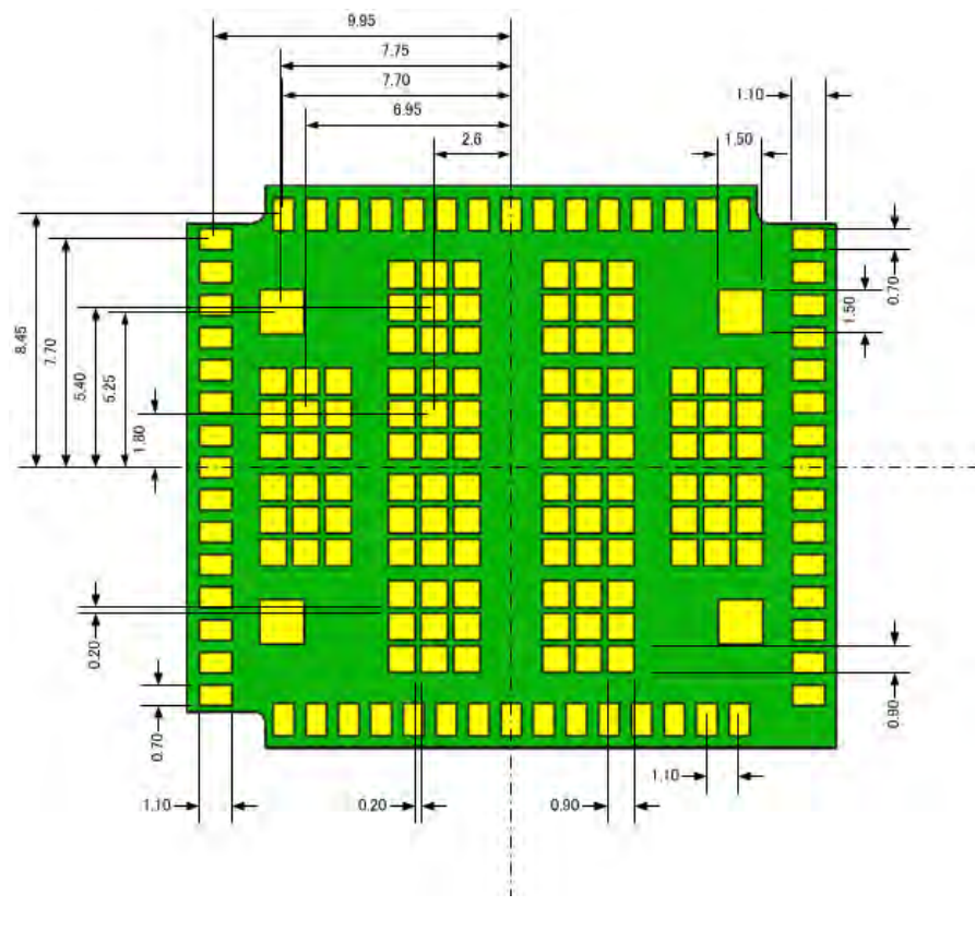
SX-SDMAC-2831S (Bottom view)
