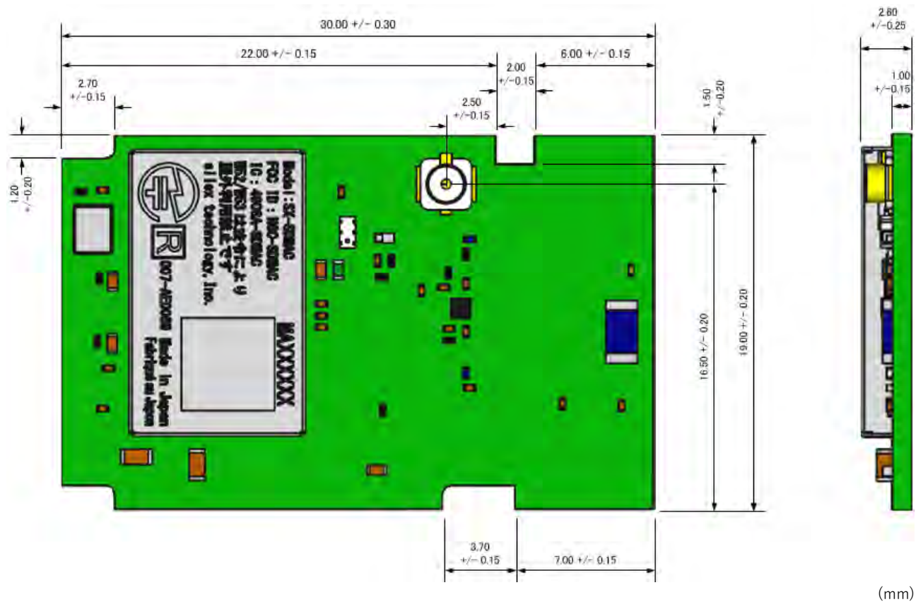
SX-SDMAC-2830S (Top view)
