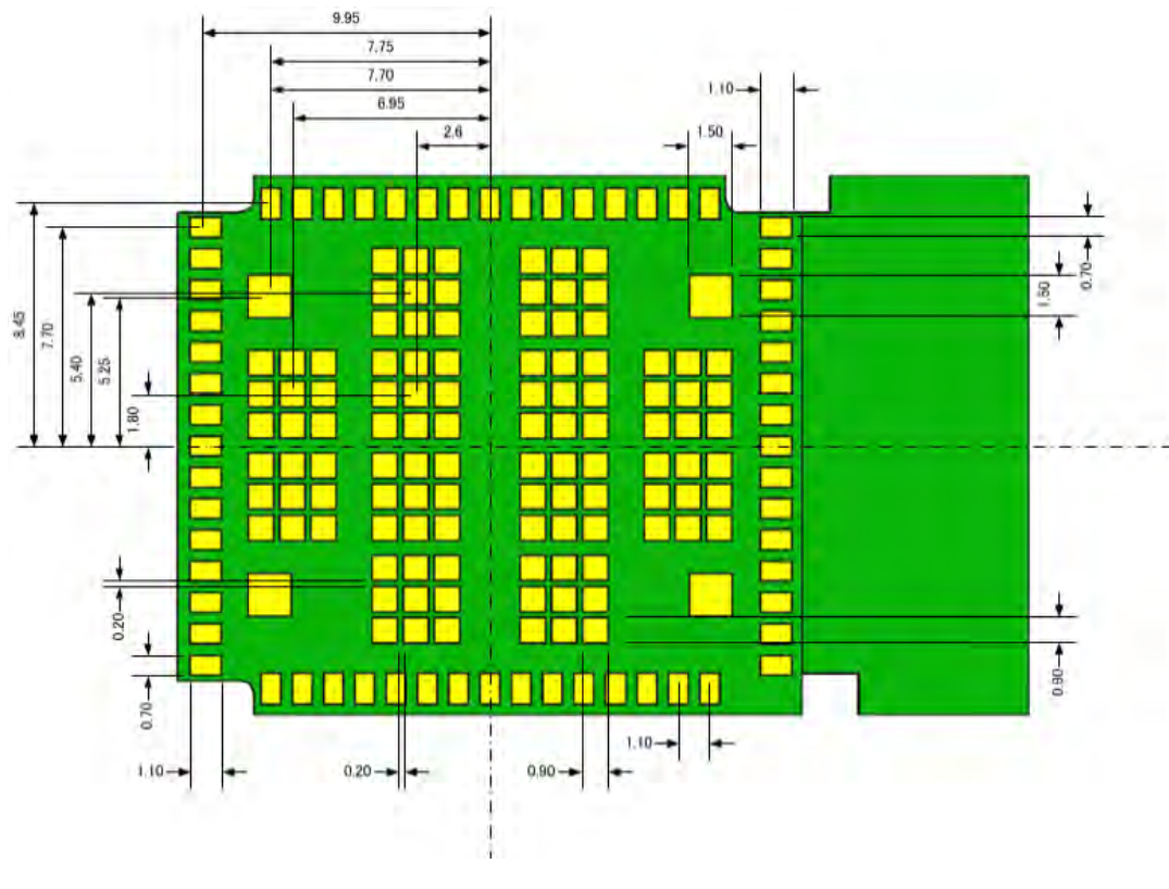
SX-SDMAC-2830S (Bottom view)
