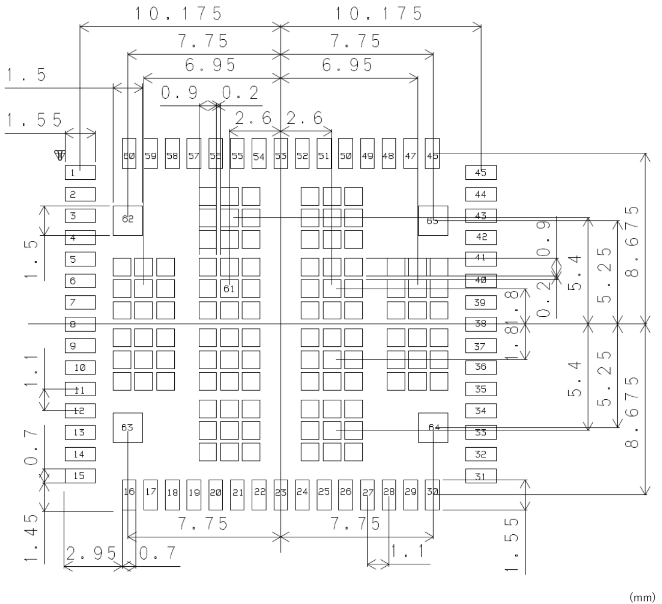
SX-SDMAC-2830S/SX-SDMAC-2831S Exposed PAD (Top View)
