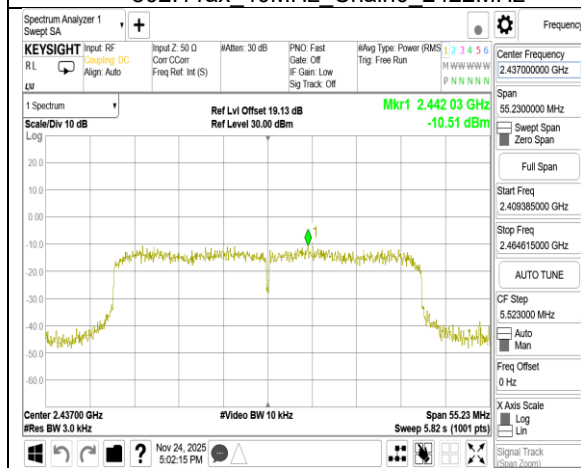
802.11ax_40MHz_Chain0_2437MHz
