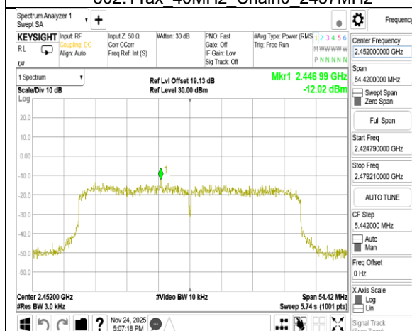
802.11ax_40MHz_Chain0_2452MHz
