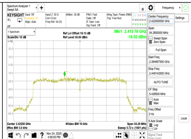
802.11ax_40MHz_Chain1_2422MHz
