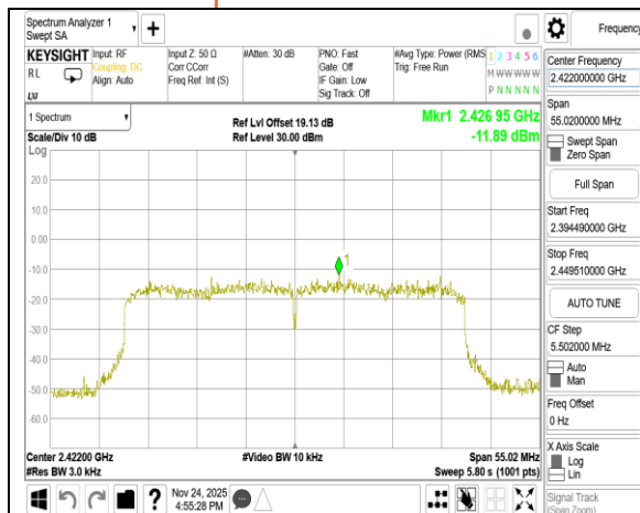
802.11ax_40MHz_Chain0_2422MHz
