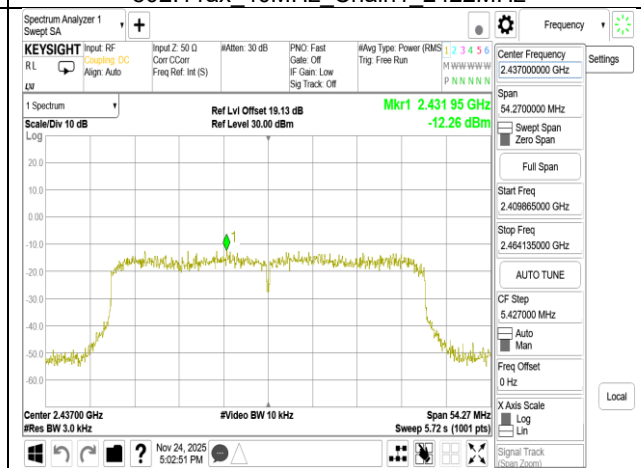
802.11ax_40MHz_Chain1_2437MHz
