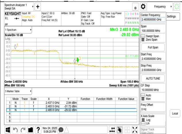
802.11ax_40MHz_Chain0_2452MHz
