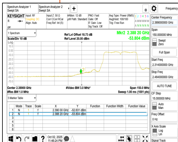
802.11n 40MHz Chain0 2432MHz
