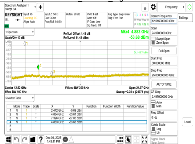
Spurious Emission_BLE 125k_MidCH20-2442MHz
