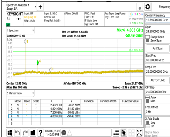
Spurious Emission_BLE 125k_LowCH00-2402MHz
