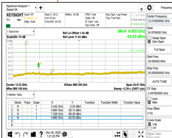
Spurious Emission_BLE 2M_MidCH20-2442MHz
