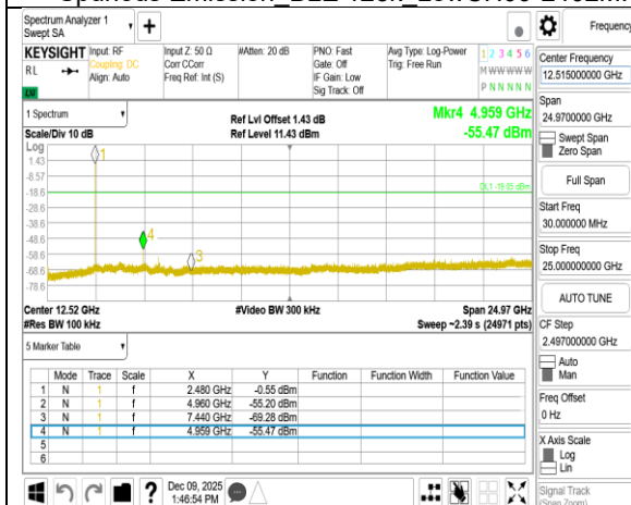
Spurious Emission_BLE 125k_HighCH39-2480MHz
