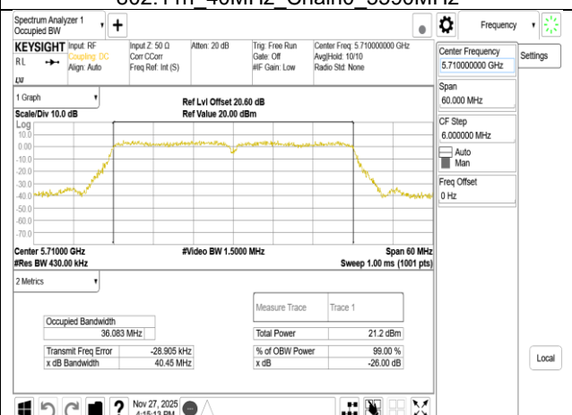
802.11n 40MHz Chain0_5710MHz
