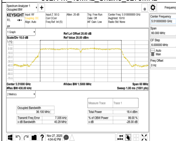
802.11n 40MHz Chain0_5510MHz
