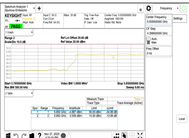
802.11n 40MHz Chain1 5835MHz UNII 2C
