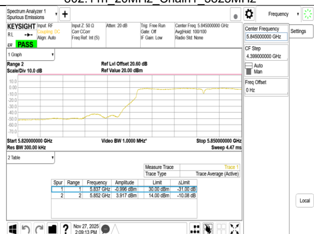
802.11n_20MHz_Chain1_5845MHz_UNII 2C
