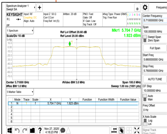
802.11n 40MHz Chain1 5710MHz UNII 2C
