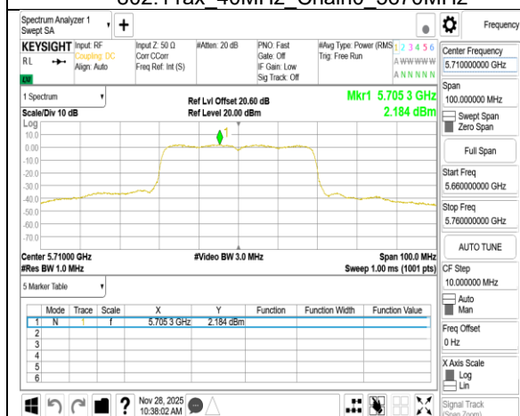
802.11ax 40MHz Chain0 5710MHz UNII 2C
