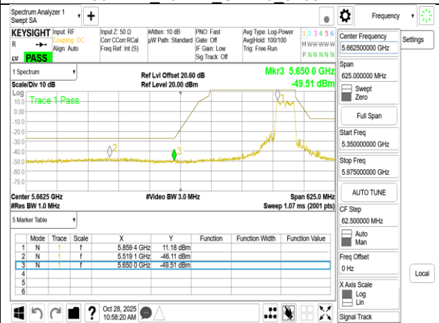
802.11n 40MHz Chain0_5875MHz
