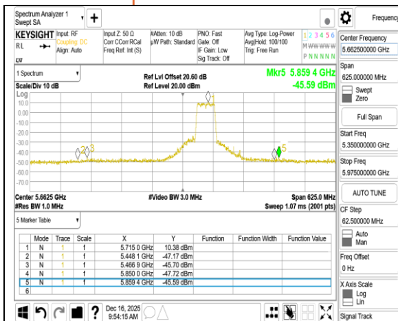
802.11n 40MHz Chain0_5710MHz
