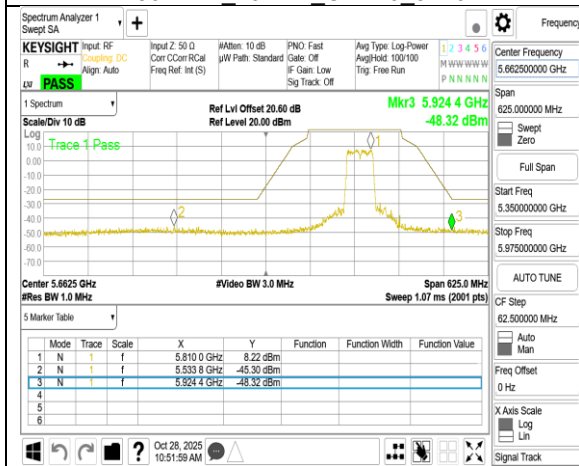
802.11n 40MHz Chain0_5795MHz
