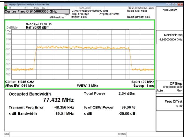
802.11ax 80MHz Chain0 6945MHz
