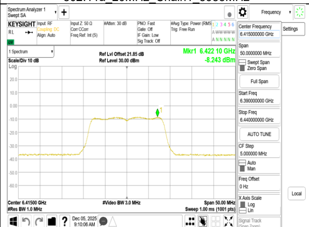
802.11a_20MHz_Chain1_6415MHz
