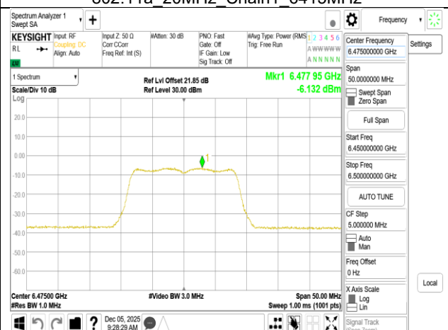
802.11a_20MHz_Chain1_6475MHz
