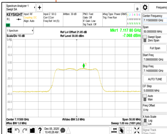
802.11a_20MHz_Chain0_7115MHz
